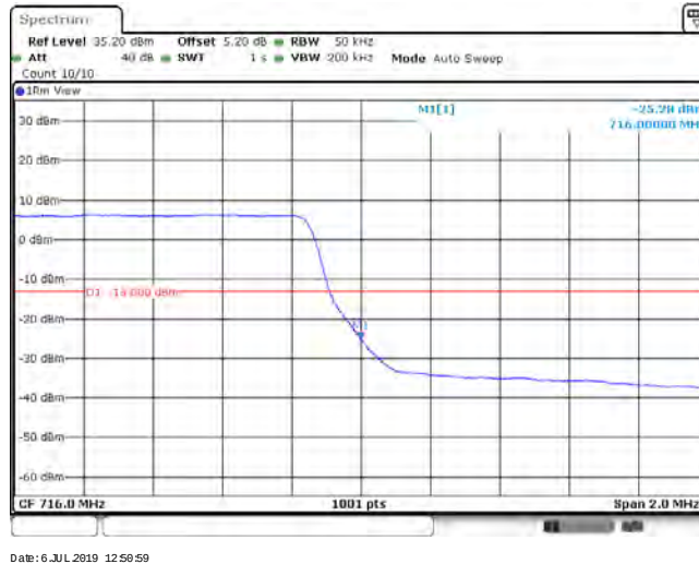
Band12_3MHz_16QAM_23025_1RB#0
