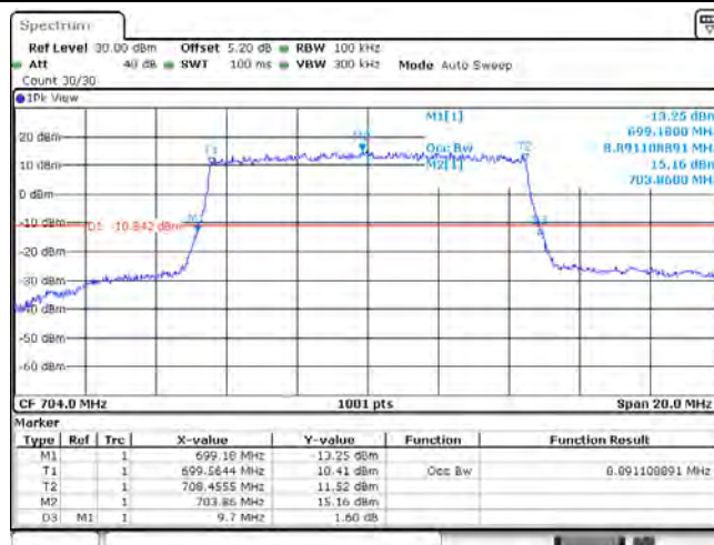
Band12_10MHz_QPSK_23095_50RB#0
