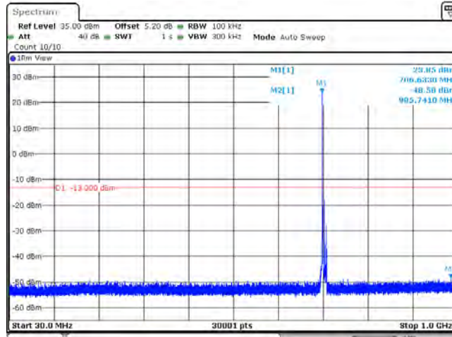
Band12_10MHz_QPSK_23130_1RB#0
