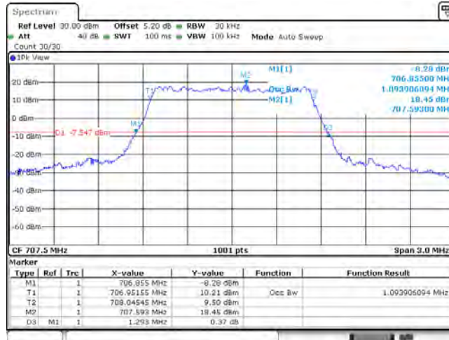
Band12_1.4MHz_QPSK_23095_6RB#0
