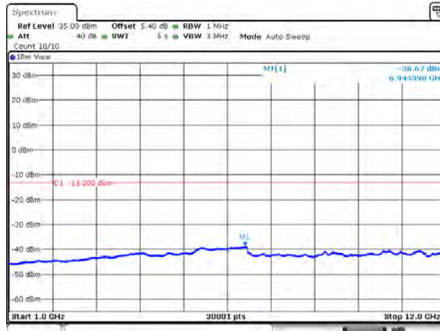
Band12_10MHz_QPSK_23130_1RB#0
