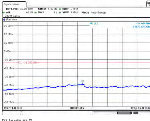
Band12_10MHz_16QAM_23130_1RB#0
