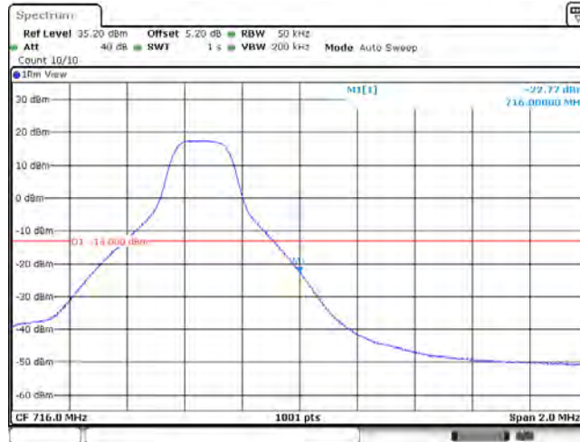
Band12_5MHz_16QAM_23155_25RB#0
