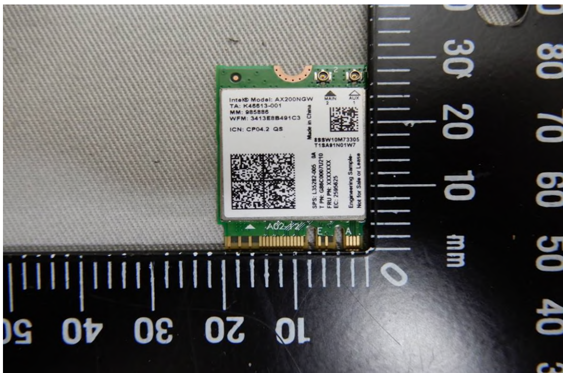
WLAN / BT Module - 1 (Model No.: AX200NGW)
