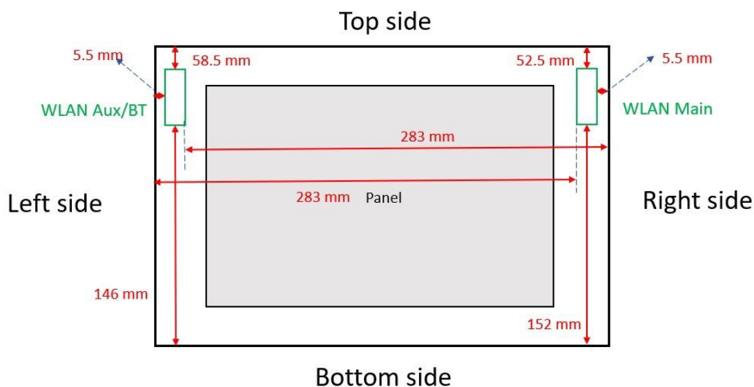
Fig.11 Antenna location of EUT (Tablet mode)
