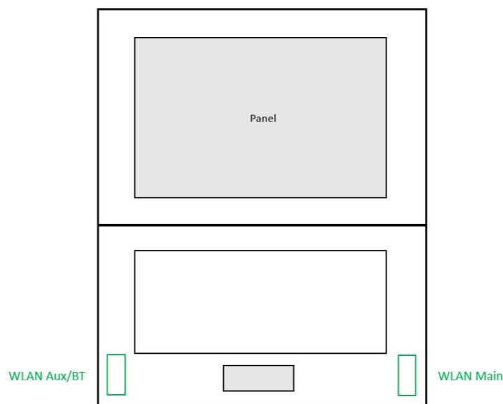
Fig.11 Antenna location of EUT (Tablet mode)
