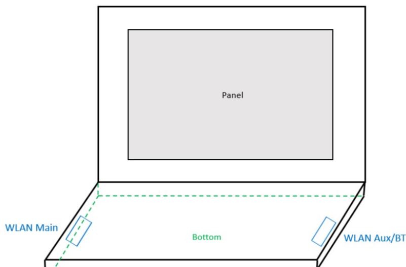
Photograph 15. Antenna position of EUT (Tablet mode)
