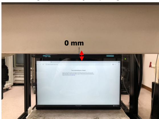
Photograph 5. Body, Bottom Edge, 0mm
