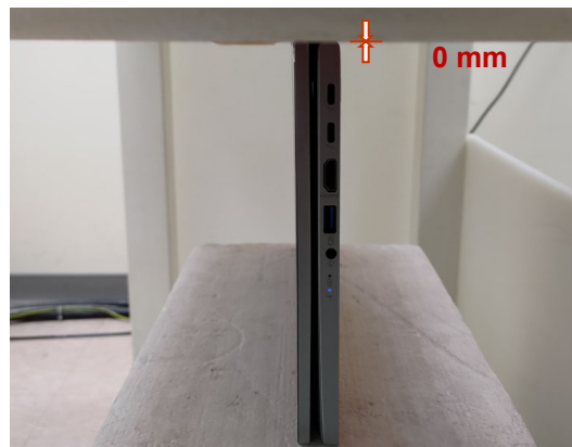
Photograph 8. Body, Bottom Edge, 0mm
