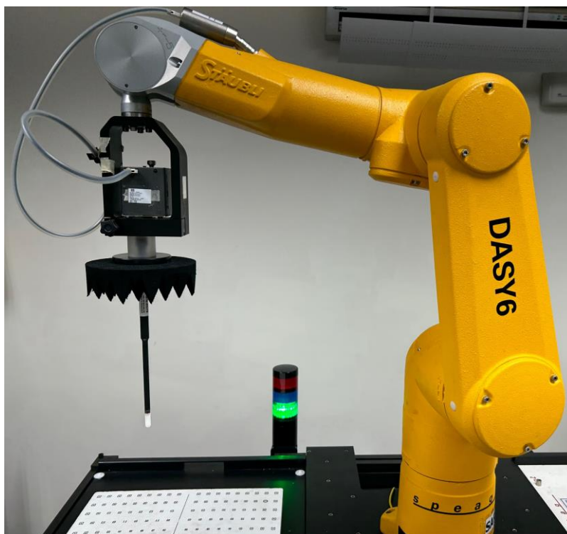
Fig.1 Photograph of the SAR/Power Density measurement system
