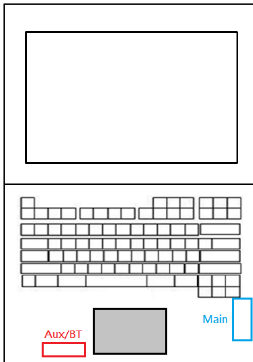
Photograph 17. Antenna position of EUT
