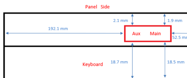
Photograph 18. Antenna position of EUT (Tablet mode)
