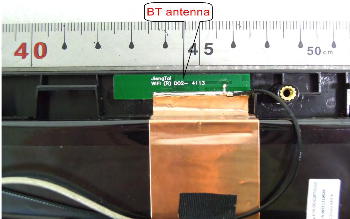
BT Antenna
