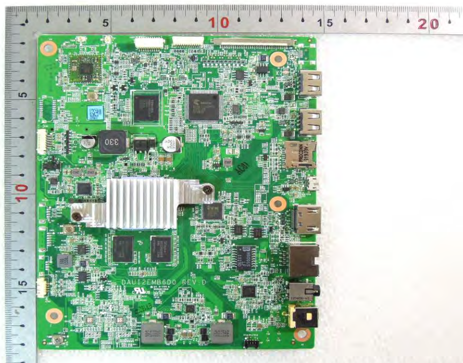
Internal View of EUT – 7
