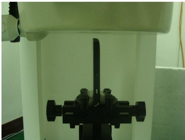
Bottom Side of the DUT with Earphone 1 cm Gap (DUT without Earphone)
