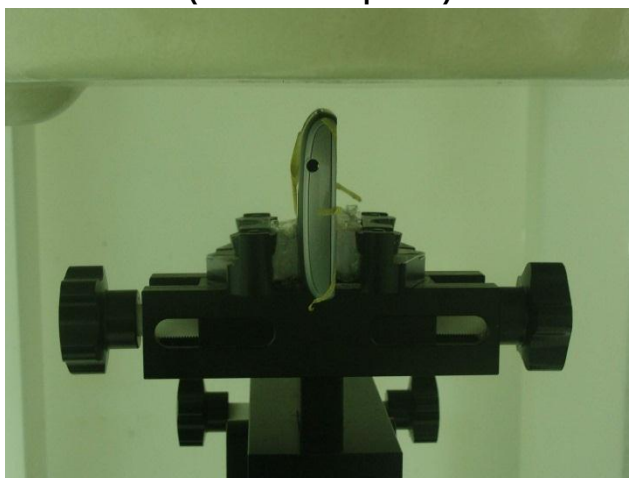
Right Side of the DUT with Phantom 1 cm Gap (DUT without Earphone)
