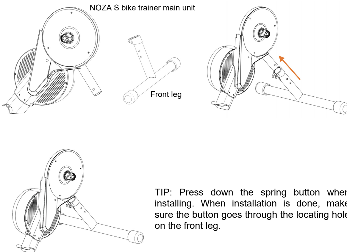
Diagram of completed front leg installation
