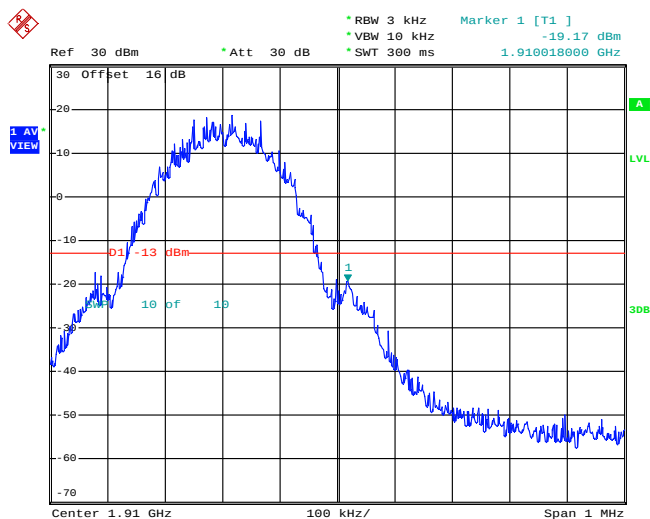
Higher Band Edge Plot on Channel 810 (1909.8 MHz)
