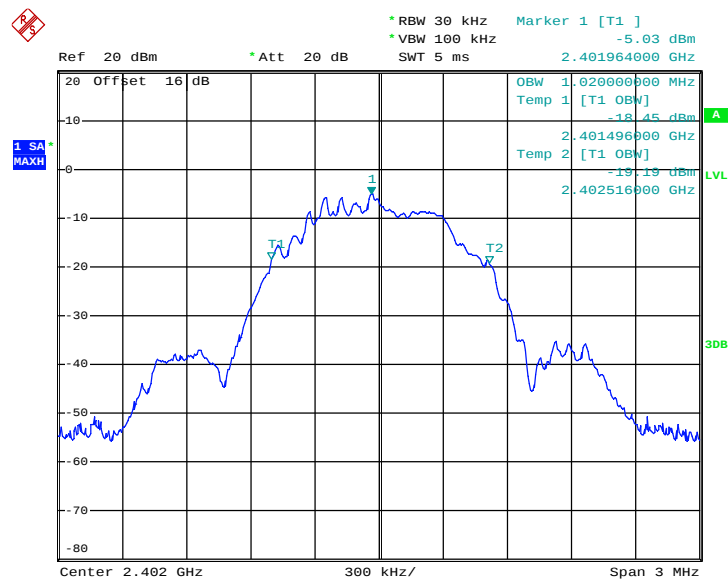
99% Bandwidth Plot on Channel 0
