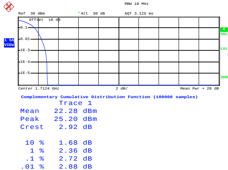
Peak-to-Average Ratio on Channel 1312 (1712.4 MHz)
