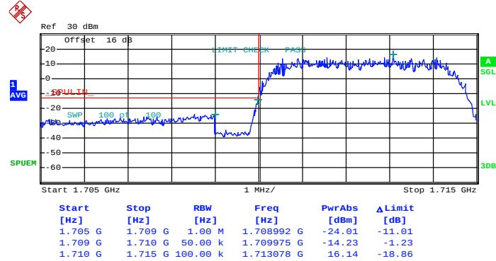
Lower Band Edge Plot on Channel 1312 (1712.4 MHz)
