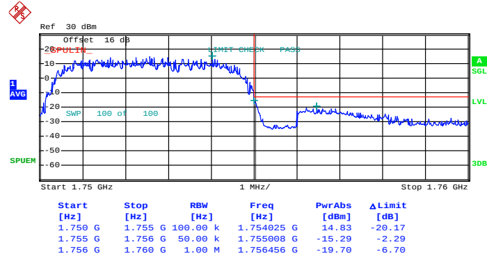
Higher Band Edge Plot on Channel 1513 (1752.6 MHz)
