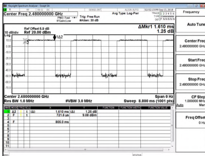
Dwell Time_8DPSK_3M_DH3_2480MHz
