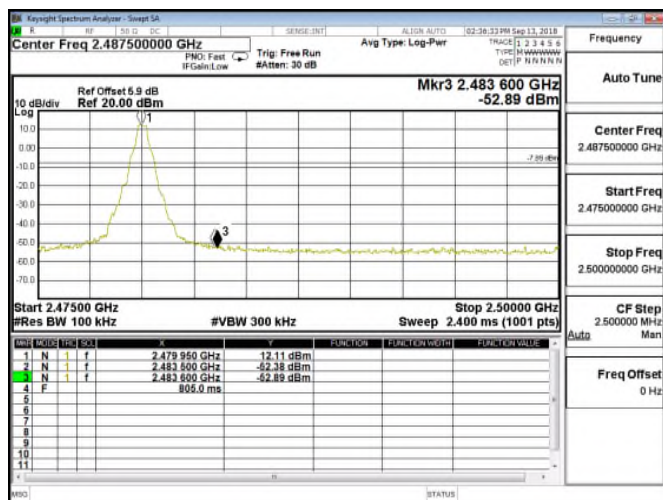
Band Edge_GFSK_1M_DH5_2480MHz
