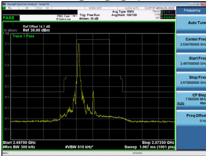
Band 7_16QAM_15M_RB1,74
