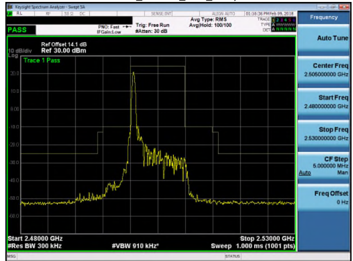
Band 7_16QAM_10M_RB1,49
