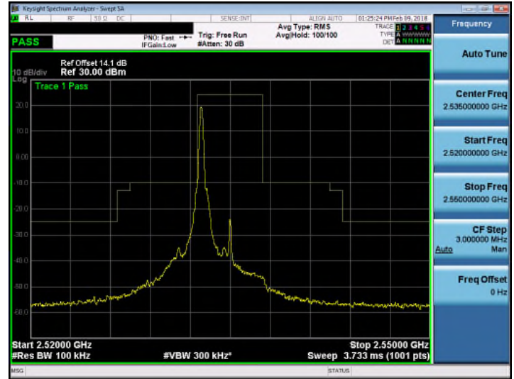
Band 7_QPSK_5M_RB1,24
