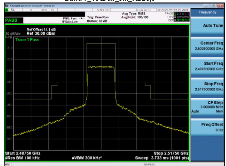
Band 7_16QAM_5M_RB25,0
