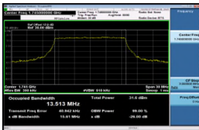
Band66_15MHz_QPSK_75_0_MidCH132322
