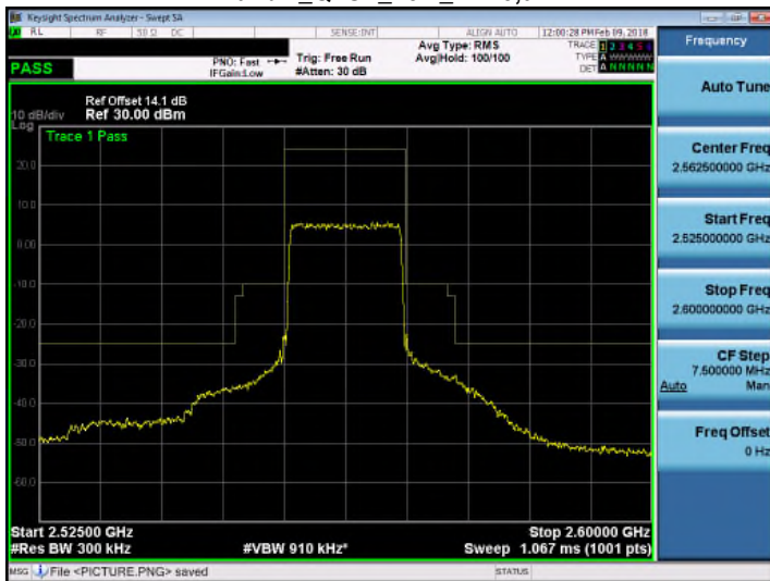
Band 7_QPSK_15M_RB75,0
