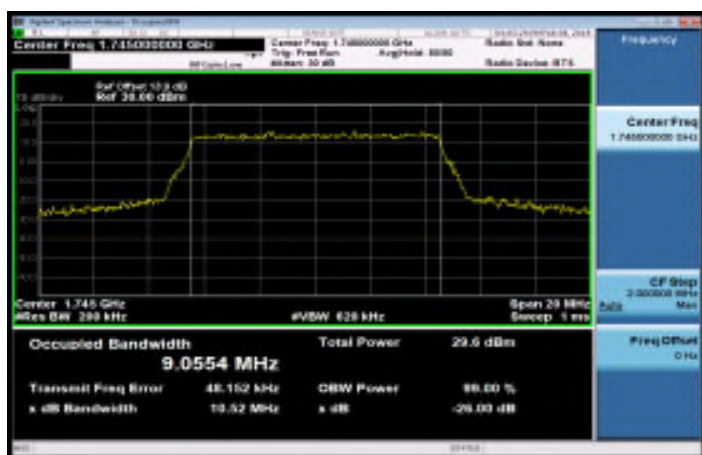
Band66_10MHz_16QAM_50_0_MidCH132322
