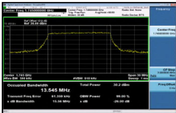
Band66_15MHz_16QAM_75_0_MidCH132322
