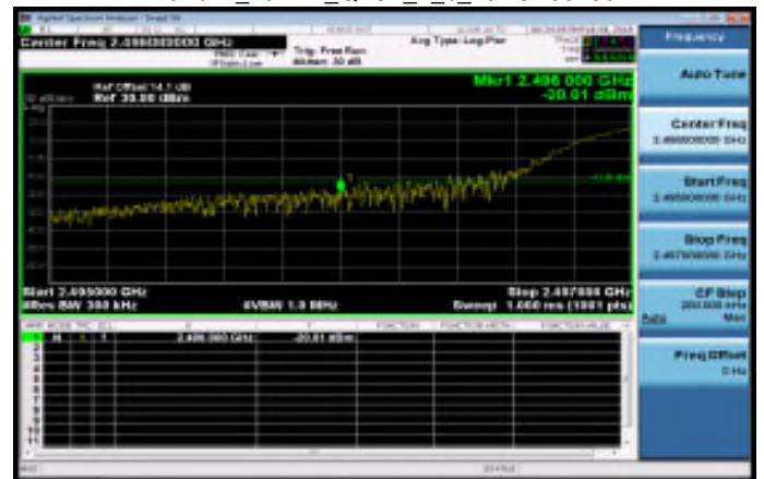
Band41_20MHz_QPSK_1_0_LowCH39750
