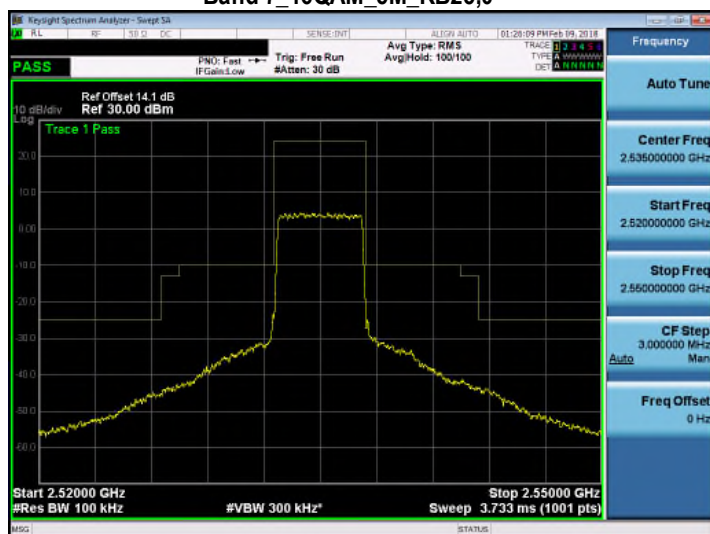
Band 7_16QAM_5M_RB25,0
