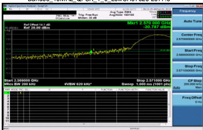
Band38_15MHz_QPSK_1_0_LowCH37825-2577.5
