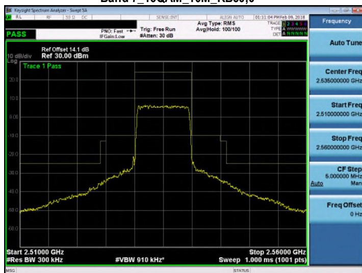
Band 7_16QAM_10M_RB50,0
