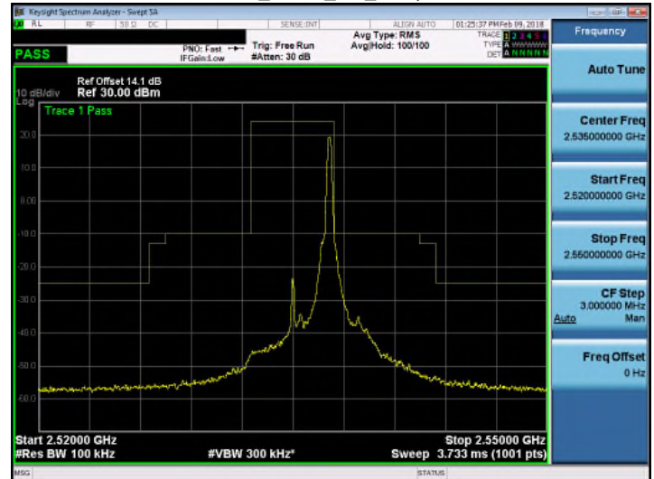
Band 7_QPSK_5M_RB25,0
