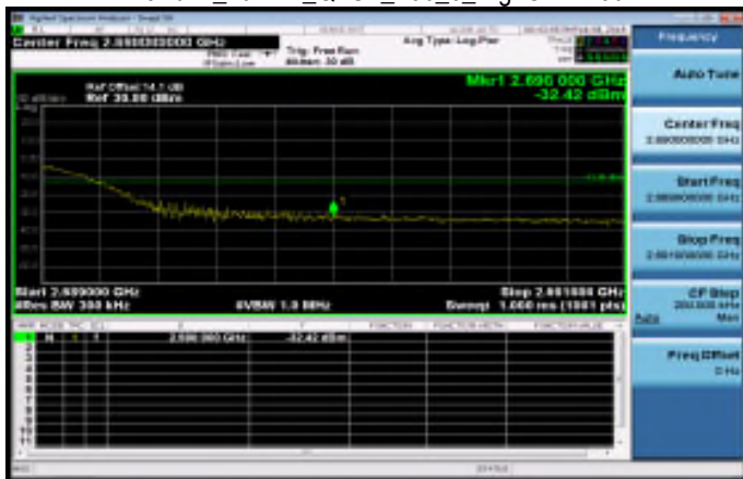
Band41_20MHz_QPSK_100_0_HighCH41490
