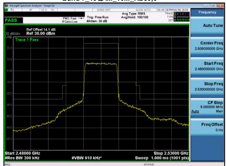
Band 7_16QAM_10M_RB50,0
