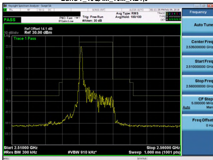
Band 7_16QAM_10M_RB1,49
