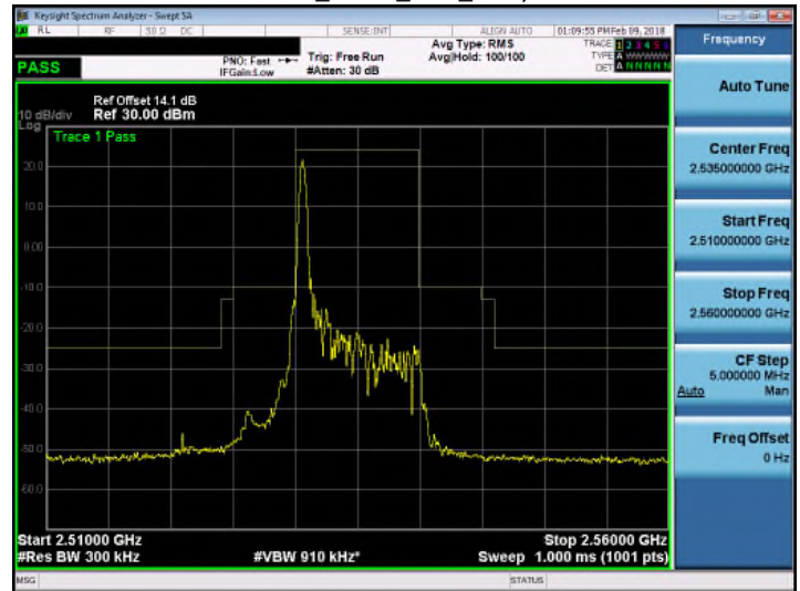
Band 7_QPSK_10M_RB1,49
