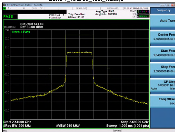
Band 7_16QAM_10M_RB50,0
