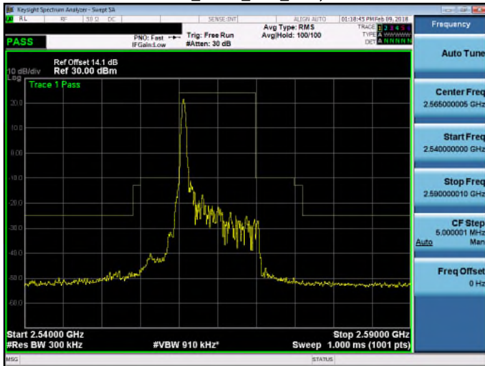
Band 7_QPSK_10M_RB1,49
