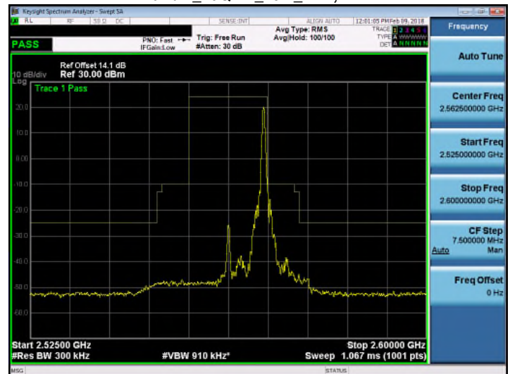
Band 7_16QAM_15M_RB75,0
