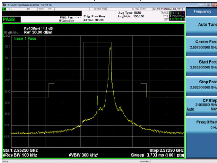
Band 7_QPSK_5M_RB25,0
