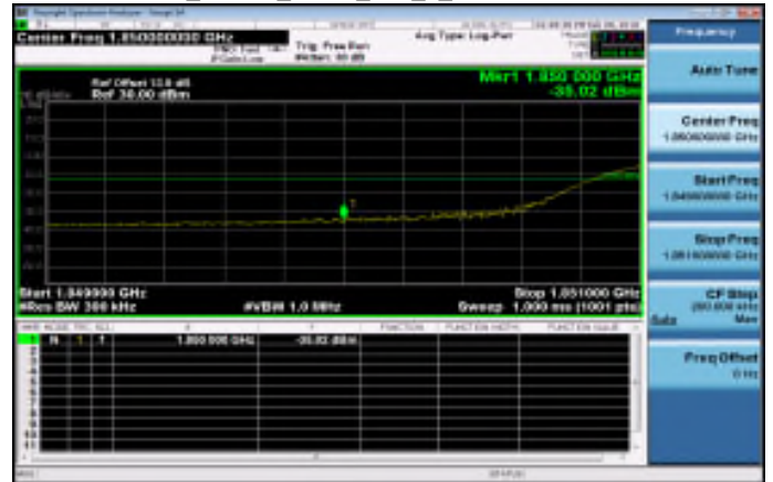
Band2_20MHz_QPSK_100_0_LowCH18700-1860
