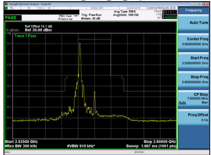
Band 7_16QAM_15M_RB1,74
