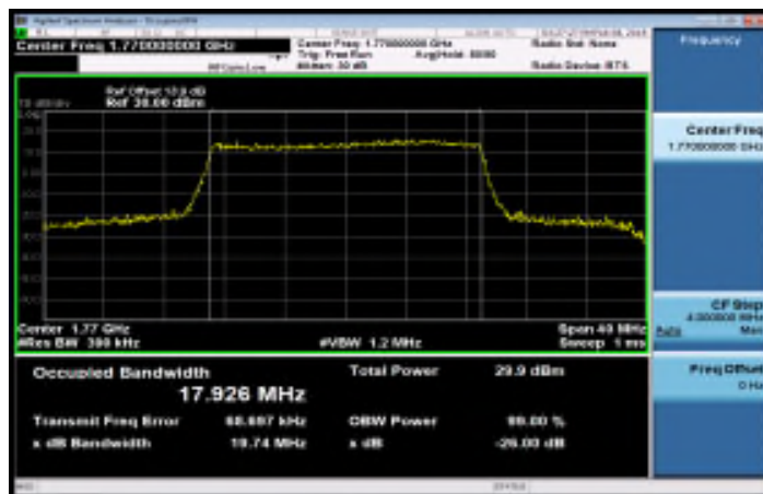
Band66_20MHz_16QAM_100_0_HighCH132572
