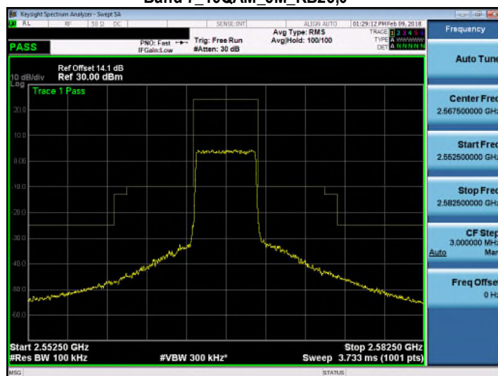
Band 7_16QAM_5M_RB25,0
