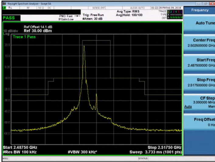
Band 7_QPSK_5M_RB1,24
