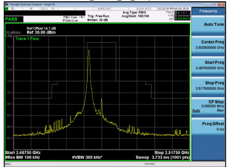
Band 7_16QAM_5M_RB1,24
