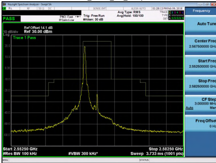
Band 7_QPSK_5M_RB1,24
