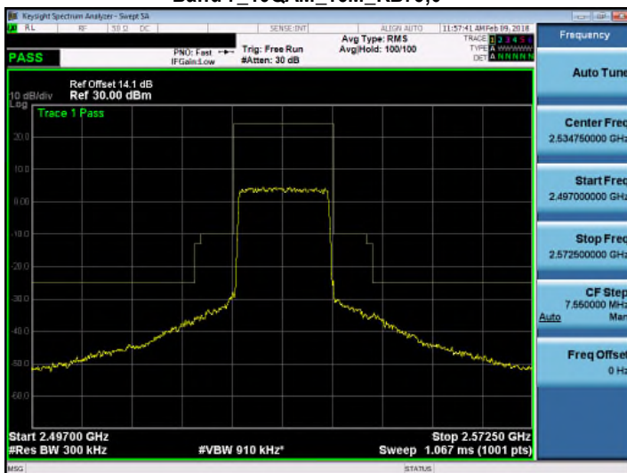
Band 7_16QAM_15M_RB75,0
