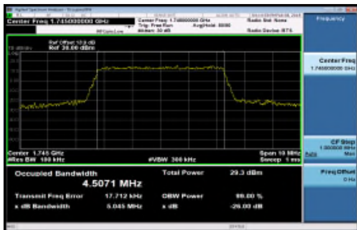
Band66_5MHz_16QAM_25_0_MidCH132322
