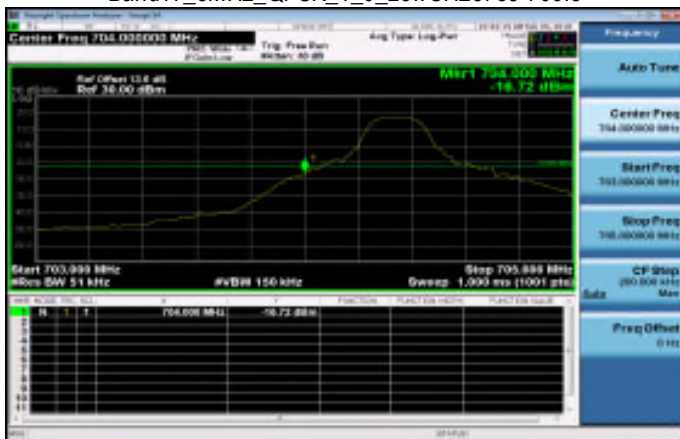
Band17_5MHz_QPSK_1_0_LowCH23755-706.5
