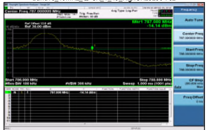
Band13_10MHz_QPSK_1_49_HighCH23230-782
