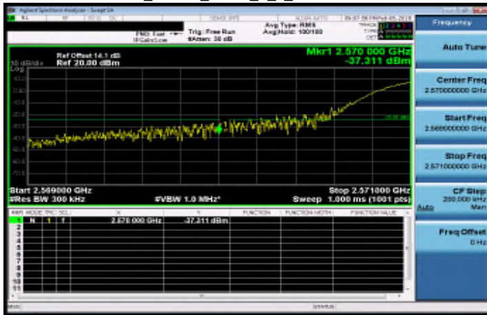
Band38_20MHz_QPSK_1_0_LowCH37850
