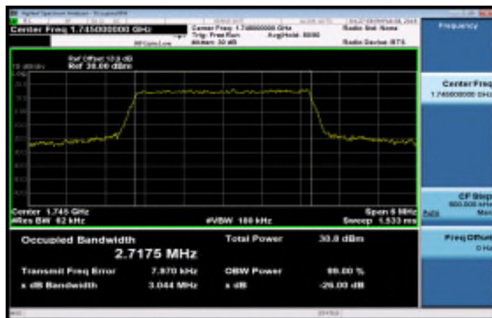
Band66_3MHz_QPSK_15_0_MidCH132322
