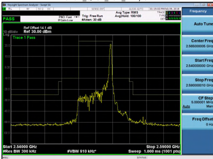
Band 7_QPSK_10M_RB50,0
