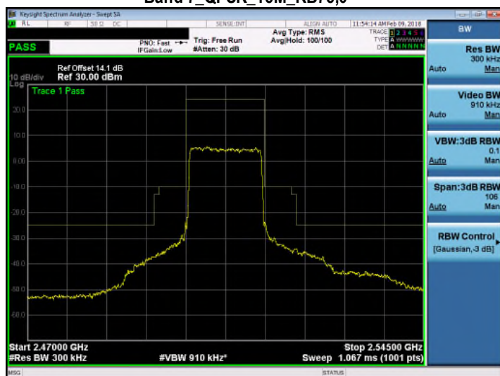
Band 7_QPSK_15M_RB75,0
