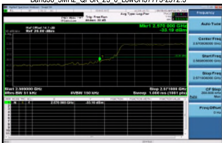
Band38_5MHz_QPSK_25_0_LowCH37775-2572.5
