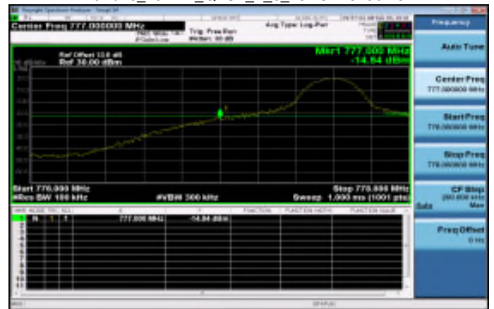
Band13_10MHz_QPSK_1_0_LowCH23230-782
