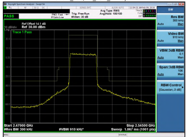
Band 7_16QAM_15M_RB75,0
