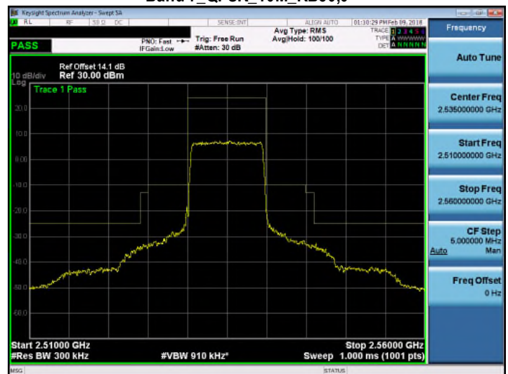
Band 7_QPSK_10M_RB50,0
