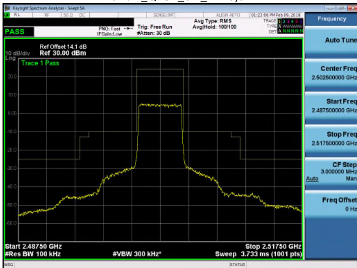
Band 7_QPSK_5M_RB25,0
