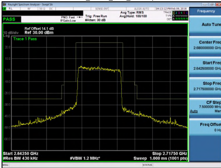
Band 41_16QAM_20M_RB1,0
