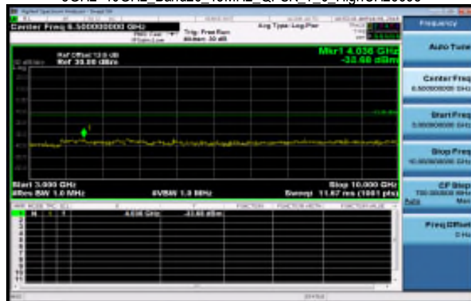
3GHz~10GHz_Band26_15MHz_QPSK_1_0_HighCH26965
