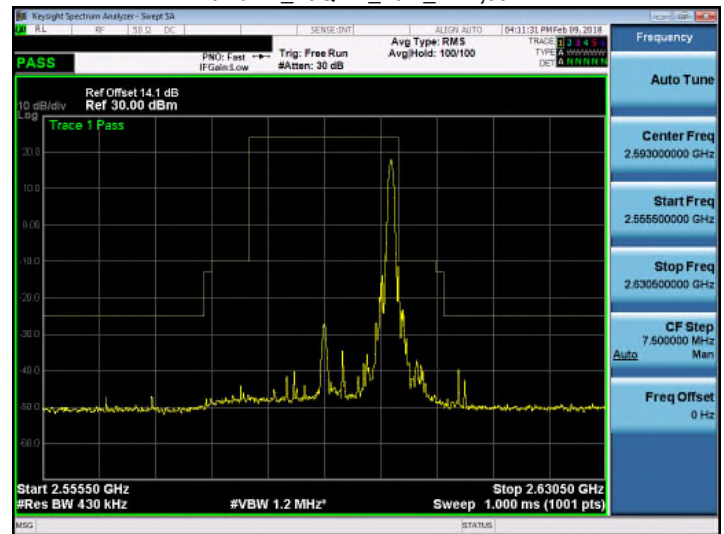
Band 41_16QAM_20M_RB1,99
