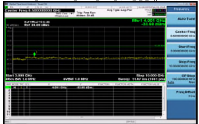
Part90_3GHz~10GHz_Band26_5MHz_QPSK_1_0_HighCH26765
