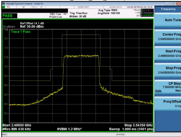
Band 41_QPSK_20M_RB1,0
