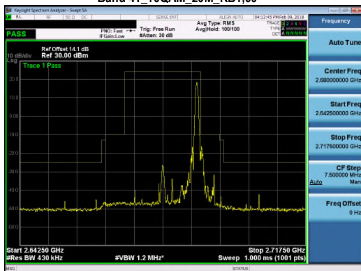
Band 41_16QAM_20M_RB1,99
