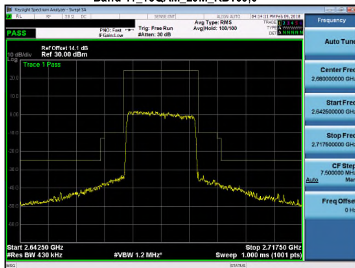
Band 41_16QAM_20M_RB100,0
