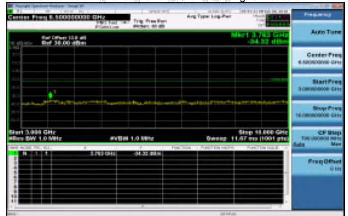
3GHz~10GHz_Band5_10MHz_QPSK_1_0_HighCH20600-844
