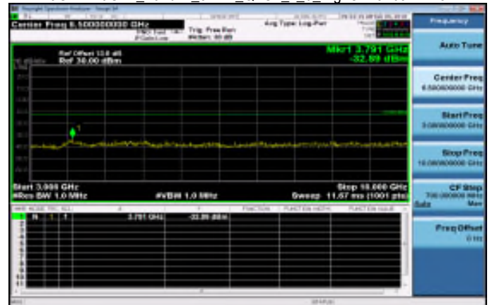
3GHz~10GHz_Band12_3MHz_QPSK_1_0_HighCH23165-714.5
