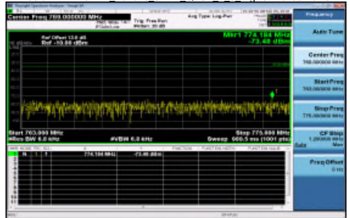
763.3MHz~775MHz Band13 5MHz QPSK 1_0 HighCH23255-784.5
