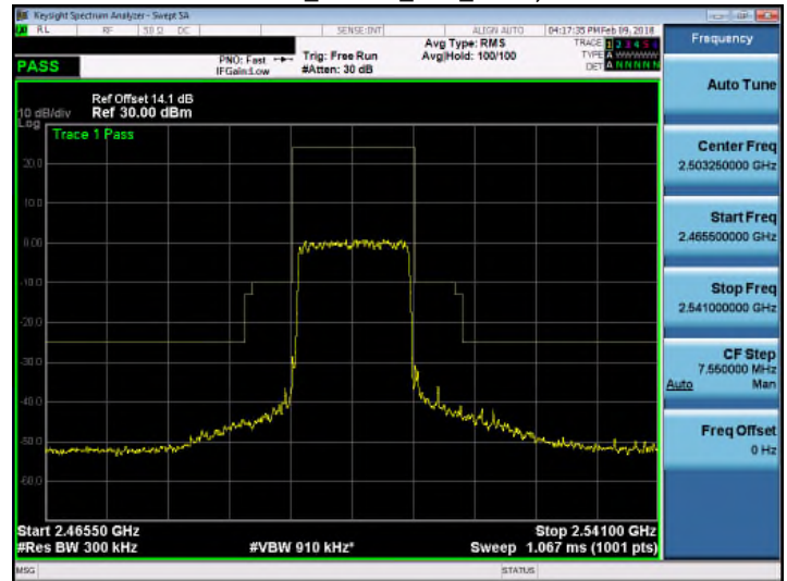
Band 41_16QAM_15M_RB1,0
