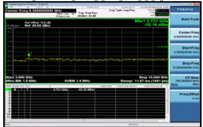
Part90 3GHz~10GHz_Band26_1_4MHz_QPSK_1_0_HighCH26783
