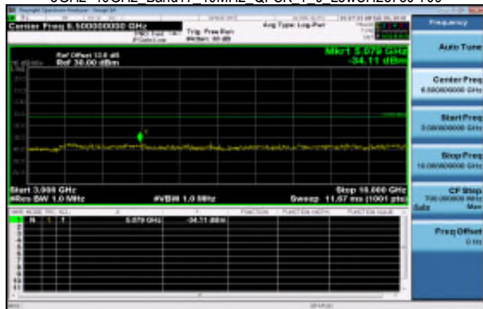
3GHz~10GHz_Band17_10MHz_QPSK_1_0_LowCH23780-709
