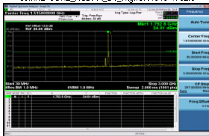
30MHz~3GHz_HSDPA_B4_HighCH1513-1752.6
