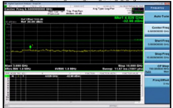
Part90_3GHz~10GHz_Band26_3MHz_QPSK_1_0_HighCH26775
