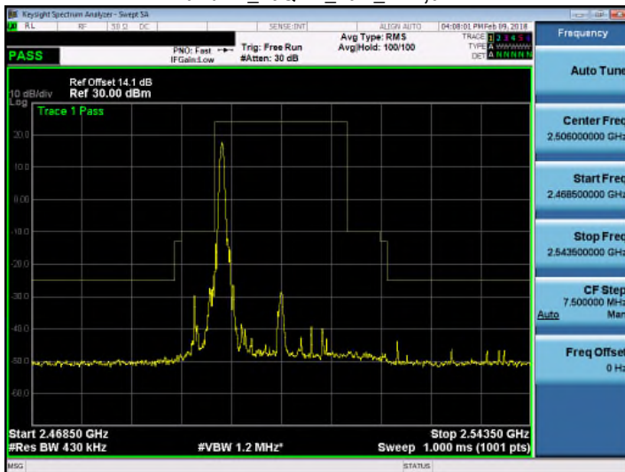
Band 41_16QAM_20M_RB1,99
