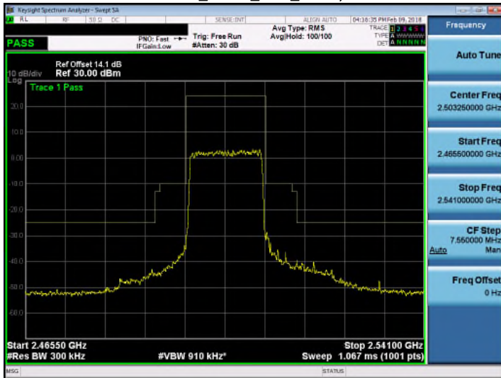
Band 41_QPSK_15M_RB1,0
