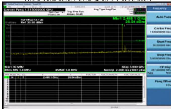
30MHz~3GHz_Band41_5MHz_QPSK_1_0_LowCH39675
