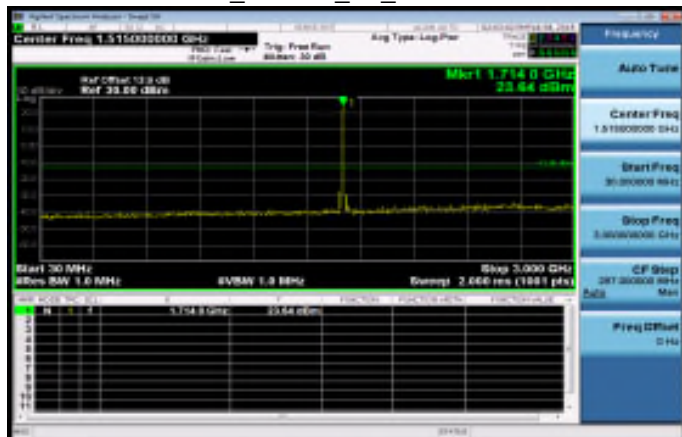
30MHz~3GHz_HSDPA_B4_LowCH1312-1712.4
