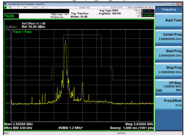
Band 41_16QAM_20M_RB1,99
