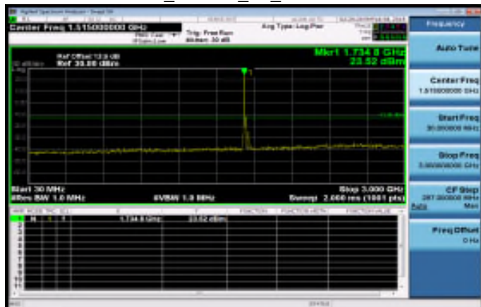
30MHz~3GHz_HSUPA_B4_MidCH1413-1732.6
