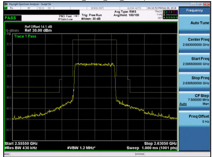
Band 41_QPSK_20M_RB1,0
