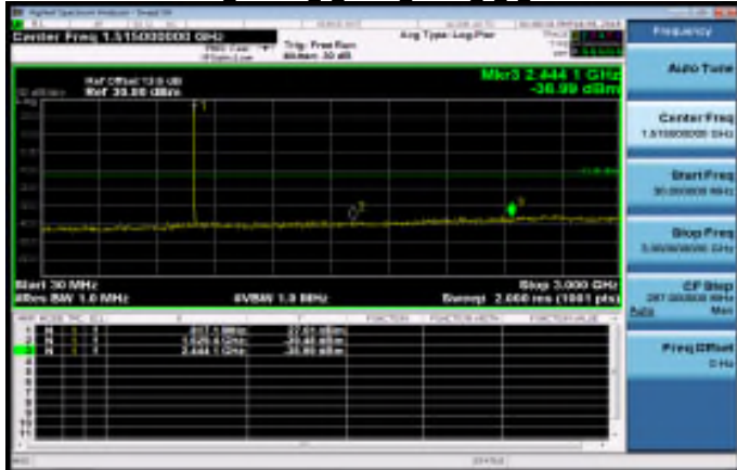
30MHz~3GHz_Band26_1_4MHz_QPSK_1_0_LowCH26697
