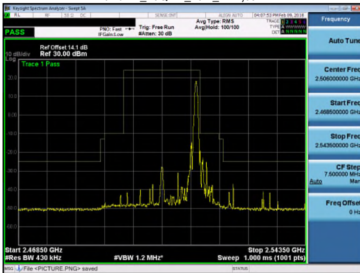
Band 41_16QAM_20M_RB1,99
