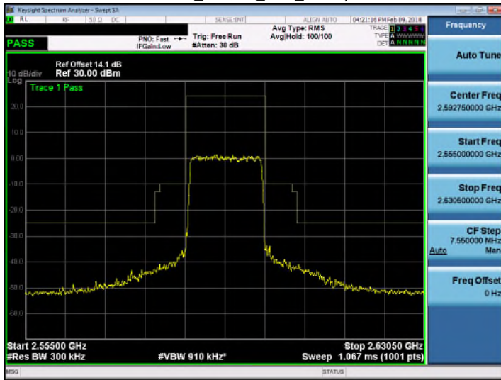
Band 41_16QAM_15M_RB1,0
