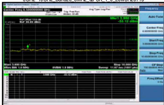
3GHz~10GHz_Band26_5MHz_QPSK_1_0_LowCH26715
