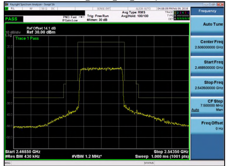
Band 41_16QAM_20M_RB1,0
