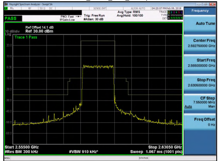
Band 41_QPSK_15M_RB1,0
