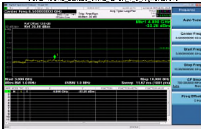
3GHz~10GHz_Band26_5MHz_QPSK_1_0_HighCH27015
