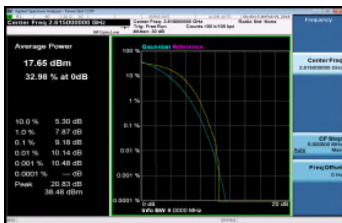
LTE_Band38_10MHz_16QAM_50_0_HighCH38200-2615
