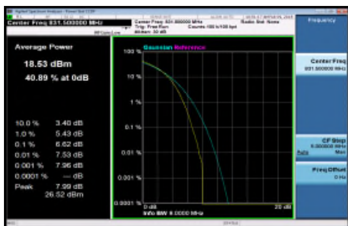
LTE_Band26_15MHz_16QAM_75_0_MidCH26865
