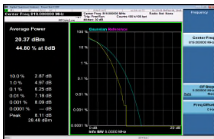
Part 90_LTE_Band26_5MHz_16QAM_25_0_MidCH26740
