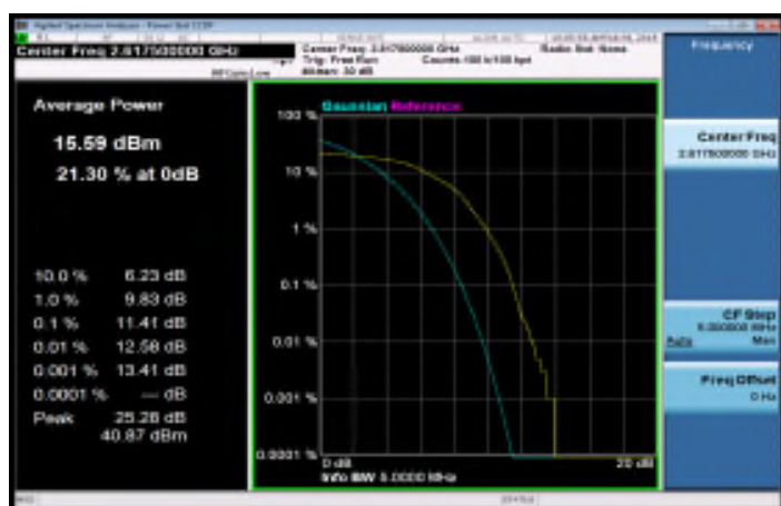
LTE_Band38_5MHz_16QAM_25_0_HighCH38225-2617.5
