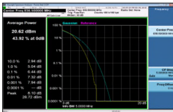
LTE_Band5_5MHz_16QAM_25_0_HighCH20625-846.5
