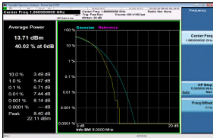
LTE_Band2_20MHz_16QAM_100_0_MidCH18900-1880
