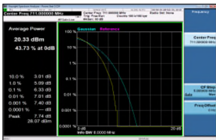
LTE_Band12_10MHz_16QAM_50_0_HighCH23130-711
