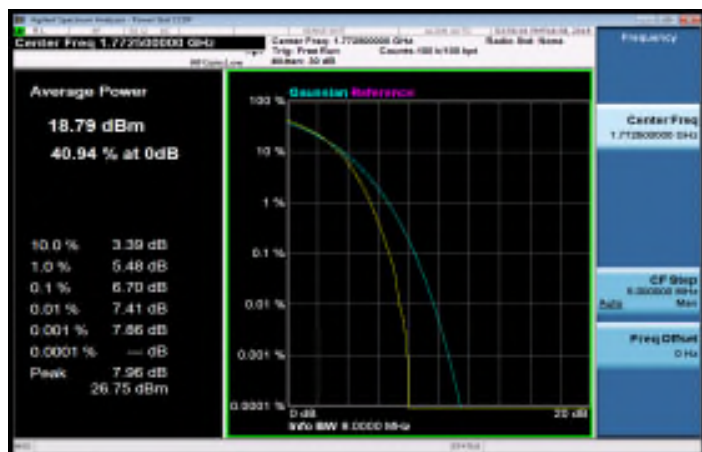
LTE_Band66_15MHz_16QAM_75_0_HighCH132597
