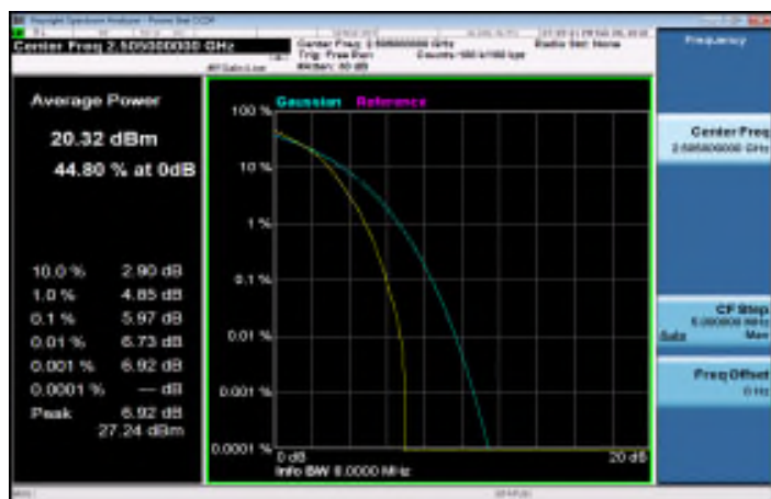
LTE_Band7_10MHz_16QAM_50_0_MidCH21100-2535
