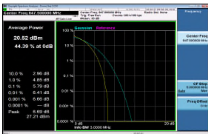
LTE_Band5_3MHz_16QAM_15_0_HighCH20635-847.5
