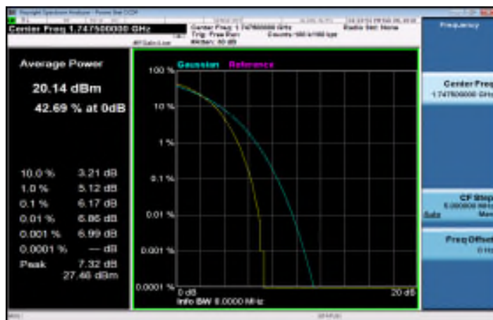
LTE_Band4_15MHz_16QAM_75_0_HighCH20325-1747.5
