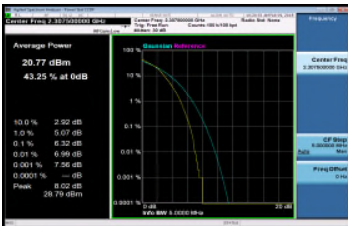
LTE_Band30_5MHz_16QAM_25_0_LowCH27685
