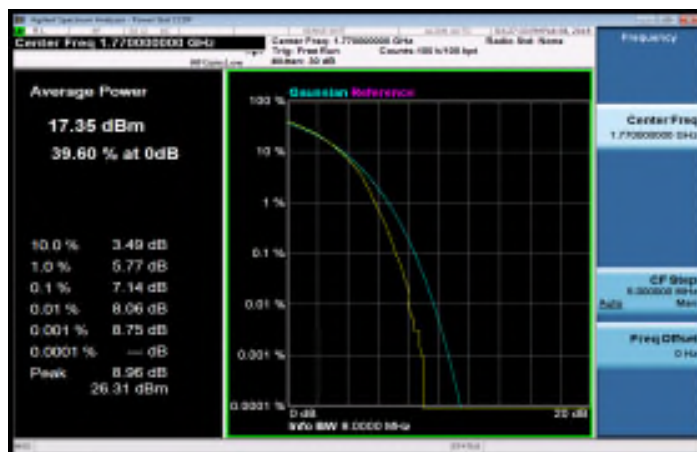
LTE_Band66_20MHz_16QAM_100_0_HighCH132572
