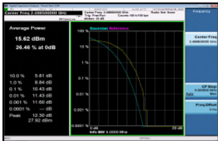
LTE_Band41_5MHz_16QAM_25_0_MidCH40620
