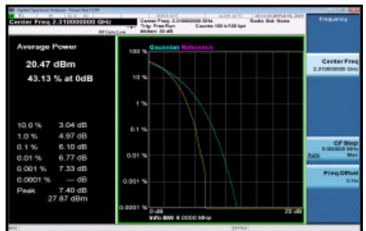
LTE_Band30_10MHz_16QAM_50_0_MidCH27710
