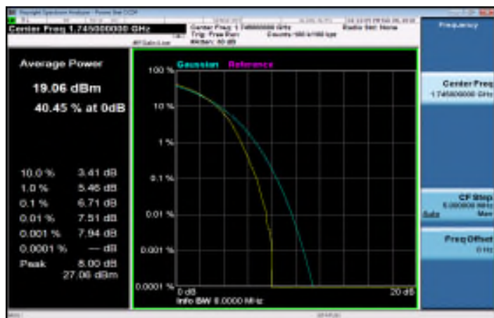
LTE_Band4_20MHz_16QAM_100_0_HighCH20300-1745
