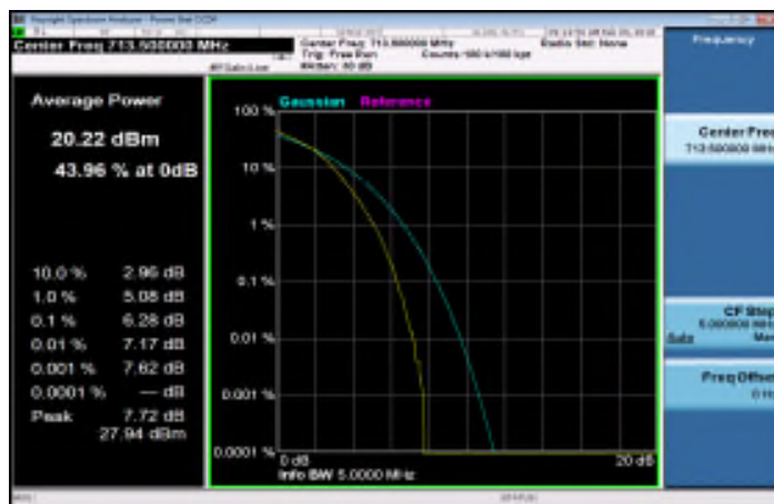
LTE_Band12_5MHz_16QAM_25_0_HighCH23155-713.5
