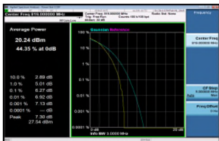
Part 90_LTE_Band26_3MHz_16QAM_15_0_MidCH26740
