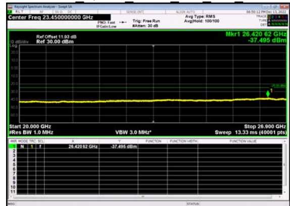
N41(80M)_DFT-s- OFDM QPSK Outer Full Mid CH
