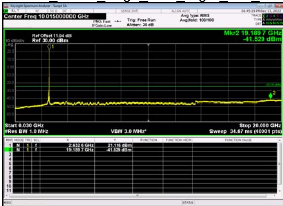
N41(80M)_DFT-s- OFDM BPSK Edge 1RB Right Mid CH
