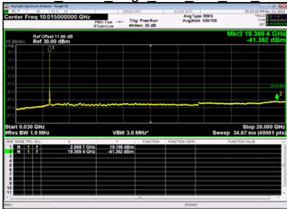
N41(50M)_DFT-s- OFDM QPSK Edge 1RB Left Mid CH
