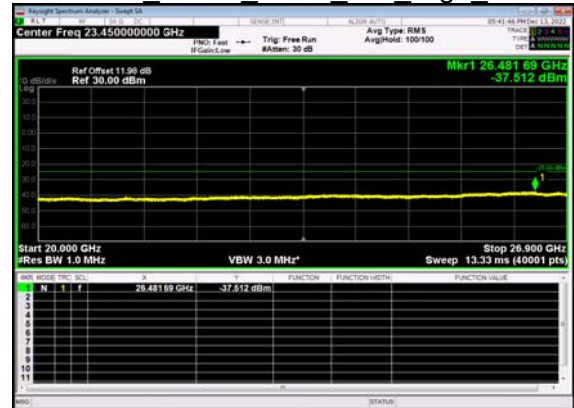
N41(40M)_DFT-s- OFDM QPSK Outer Full High CH
