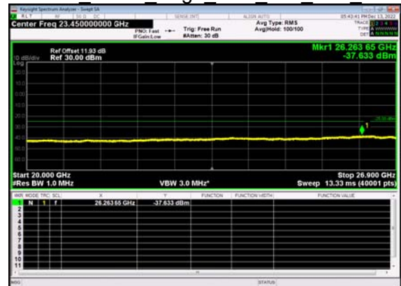
N41(50M)_DFT-s- OFDM BPSK Edge 1RB Left Low CH
