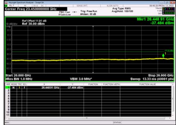
N41(80M)_DFT-s- OFDM BPSK Outer Full Low CH
