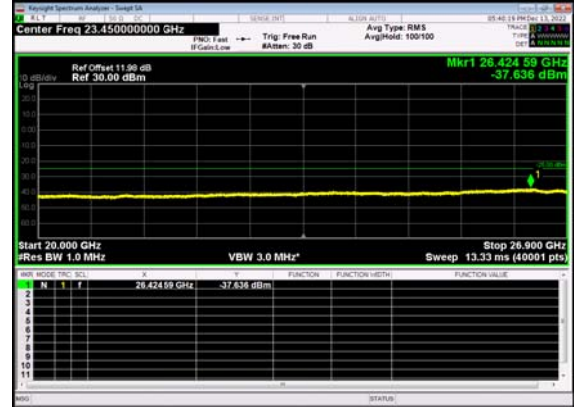
N41(40M)_DFT-s- OFDM BPSK Outer Full High CH
