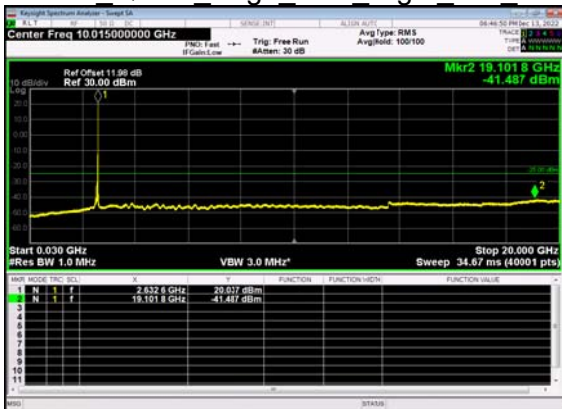
N41(80M)_DFT-s- OFDM QPSK Edge 1RB Right Mid CH
