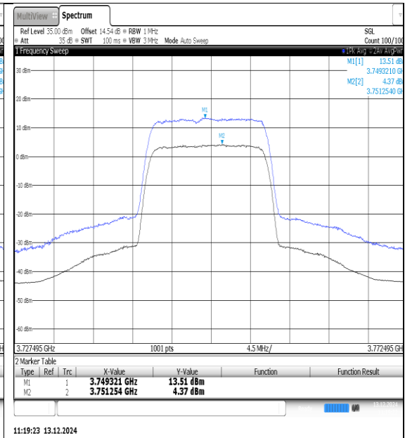
NTNV-N78-3700-3800-PC3-30-20-M-DFT-16QAM-Outet_Full-Ant1-PASS
