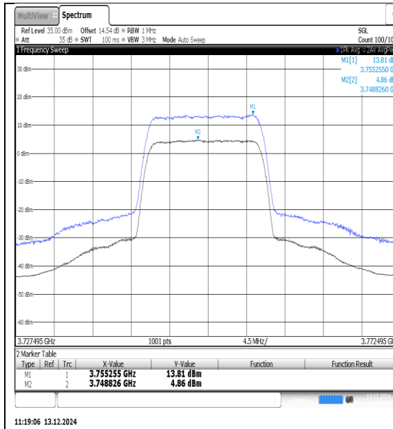
NTNV-N78-3700-3800-PC3-30-20-M-DFT-QPSK-Outet_Full-Ant1-PASS
