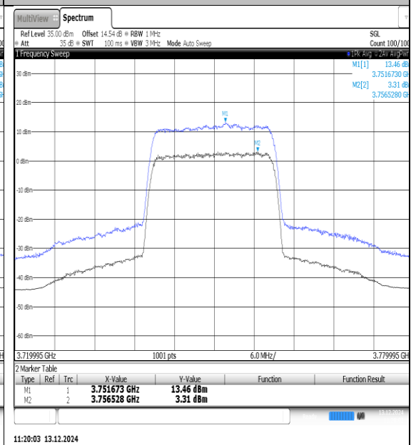
NTNV-N78-3700-3800-PC3-30-25-M-DFT-16QAM-Outet_Full-Ant1-PASS
