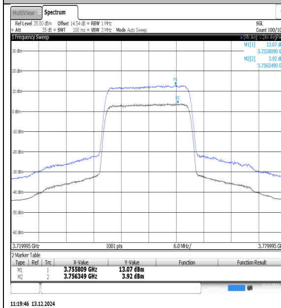
NTNV-N78-3700-3800-PC3-30-25-M-DFT-QPSK-Outet_Full-Ant1-PASS
