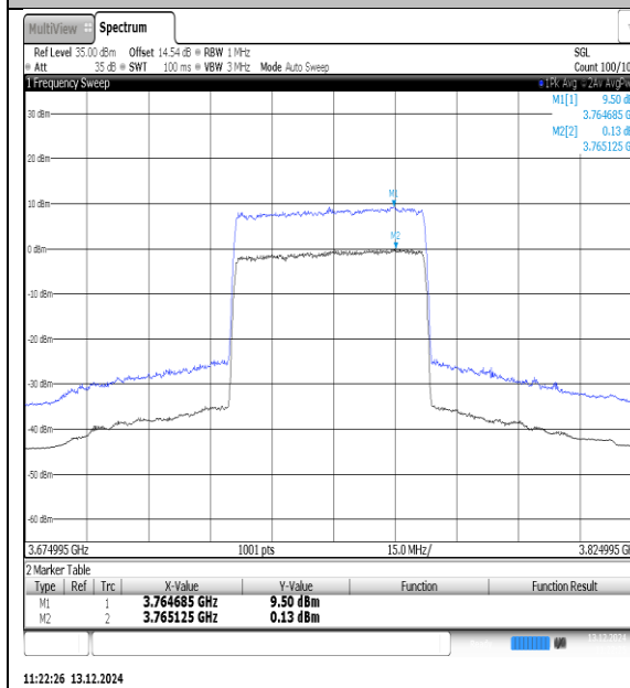
NTNV-N78-3700-3800-PC3-30-60-M-DFT-QPSK-Outet_Full-Ant1-PASS
