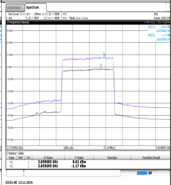
NTNV-N77-3700-3980-PC3-30-80-M-DFT-16QAM-Outet_Full-Ant1-PASS
