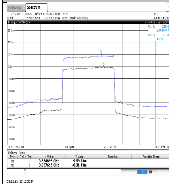
NTNV-N77-3700-3980-PC3-30-80-M-DFT-QPSK-Outet_Full-Ant1-PASS
