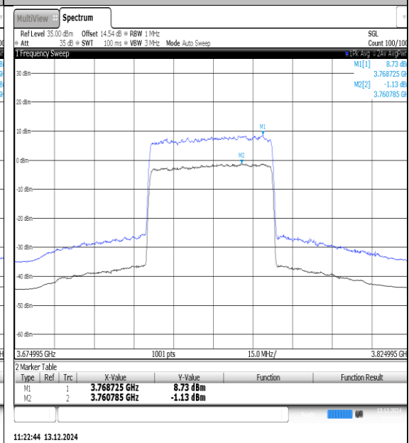
NTNV-N78-3700-3800-PC3-30-60-M-DFT-16QAM-Outet_Full-Ant1-PASS
