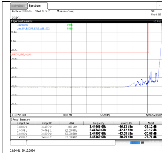
Band42(3450-3550)-5MHz-QPSK-43065-25RB#0-PASS
