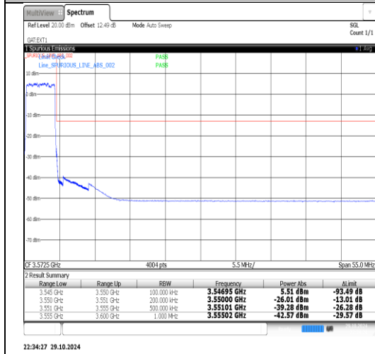
Band2(3450-3550)-10MHz-QPSK-42140-1RB#0-PASS
