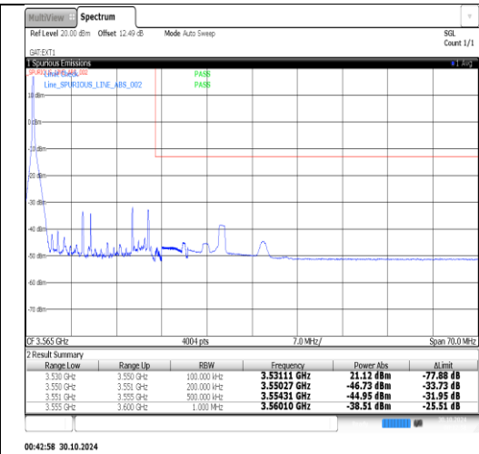
Band2(3450-3550)-20MHz-QPSK-42990-1RB#99-PASS
