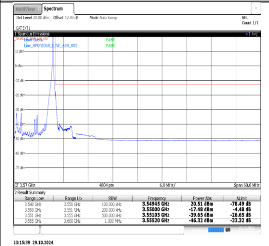
Band2(3450-3550)-10MHz-16QAM-42140-50RB#0-PASS
