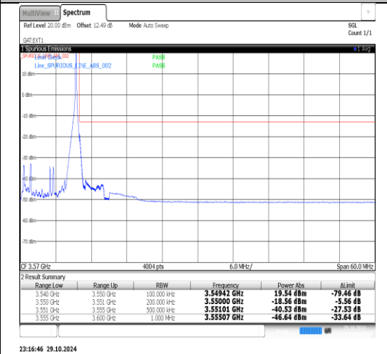
Band42(3450-3550)-15MHz-QPSK-42165-75RB#0-PASS
