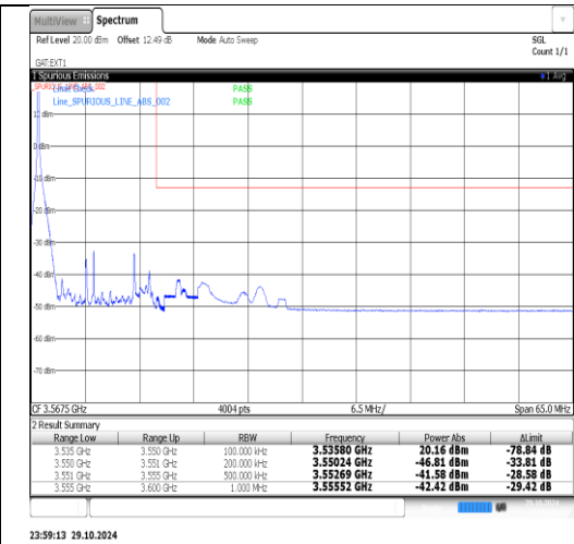
Band42(3450-3550)-15MHz-16QAM-43015-1RB#74-PASS
