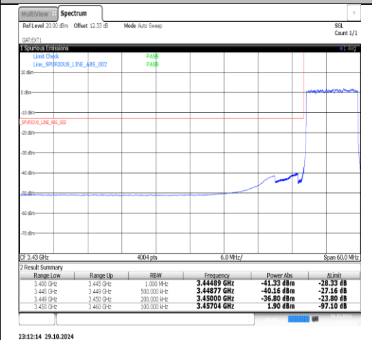
Band2(3450-3550)-10MHz-16QAM-43040-1RB#0-PASS
