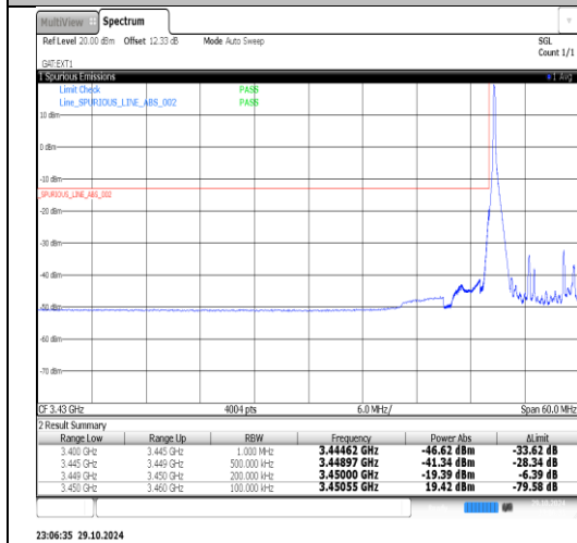
Band2(3450-3550)-10MHz-QPSK-42140-1RB#49-PASS
