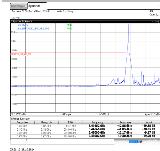
Band42(3450-3550)-15MHz-QPSK-42165-1RB#74-PASS
