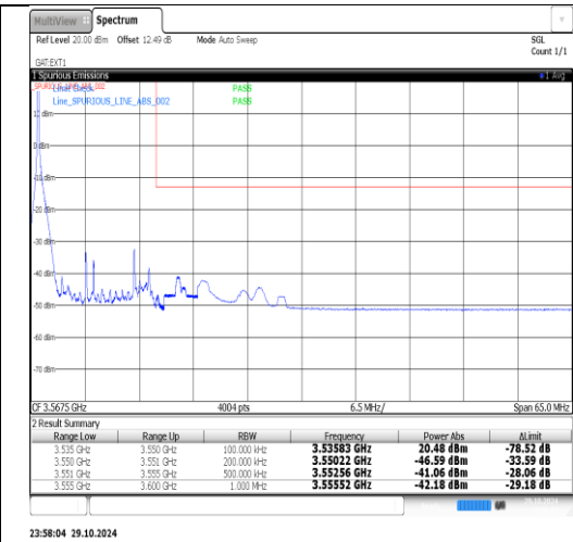
Band42(3450-3550)-15MHz-QPSK-43015-1RB#74-PASS
