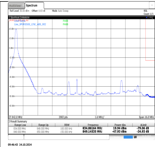
Band26(824-849)-15MHz-16QAM-26965-1RB#74-PASS
