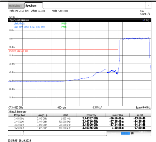
Band42(3450-3550)-15MHz-QPSK-43015-1RB#0-PASS
