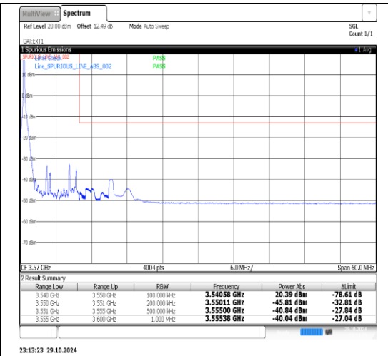
Band2(3450-3550)-10MHz-QPSK-43040-1RB#49-PASS
