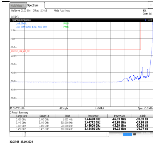
Band2(3450-3550)-5MHz-16QAM-43065-25RB#0-PASS
