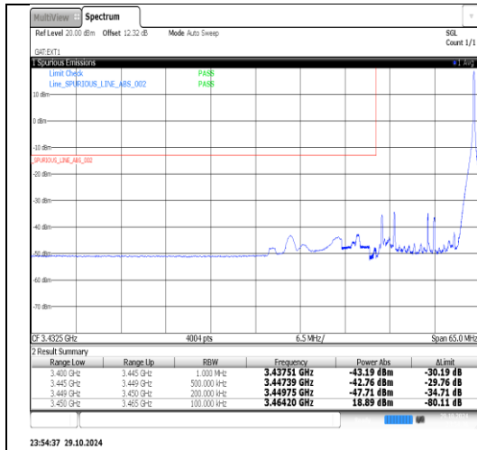
Band42(3450-3550)-15MHz-16QAM-43015-75RB#0-PASS
