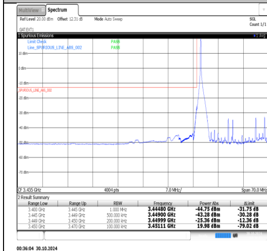
Band42(3450-3550)-20MHz-QPSK-42190-1RB#99-PASS
