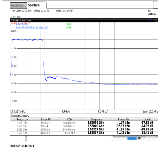
Band42(3450-3550)-20MHz-QPSK-42190-1RB#0-PASS
