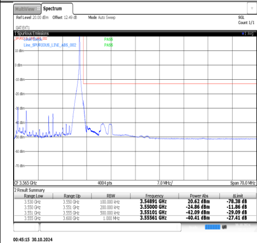
Band2(3450-3550)-20MHz-16QAM-42190-100RB#0-PASS
