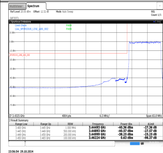
Band42(3450-3550)-15MHz-16QAM-43015-1RB#0-PASS
