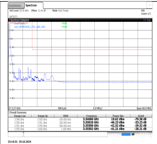
Band42(3450-3550)-10MHz-16QAM-43040-1RB#49-PASS
