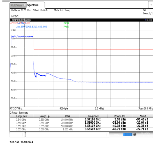
Band2(3450-3550)-10MHz-16QAM-42140-1RB#0-PASS
