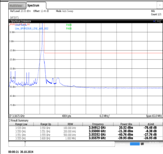
Band42(3450-3550)-15MHz-16QAM-42165-75RB#0-PASS
