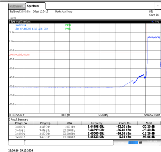
Band42(3450-3550)-5MHz-QPSK-43065-1RB#0-PASS
