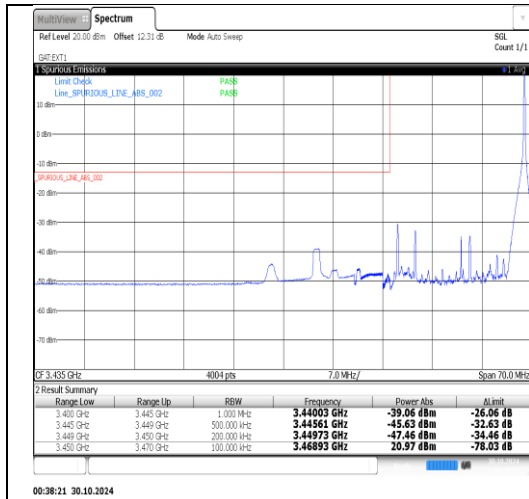
Band2(3450-3550)-20MHz-QPSK-42990-100RB#0-PASS
