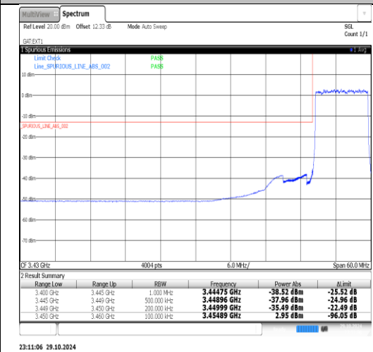
Band2(3450-3550)-10MHz-QPSK-43040-1RB#0-PASS
