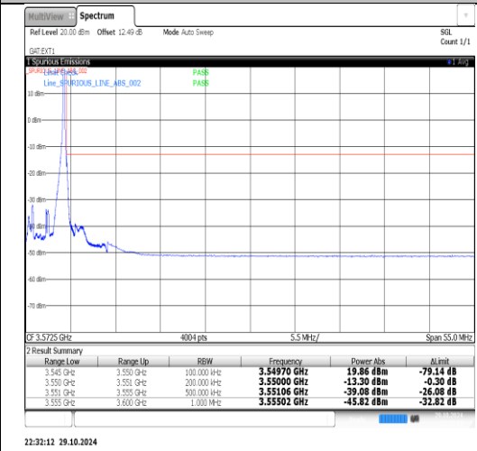
Band2(3450-3550)-10MHz-QPSK-42140-50RB#0-PASS
