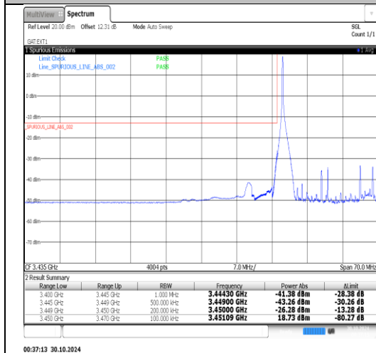
Band2(3450-3550)-20MHz-16QAM-42190-1RB#99-PASS
