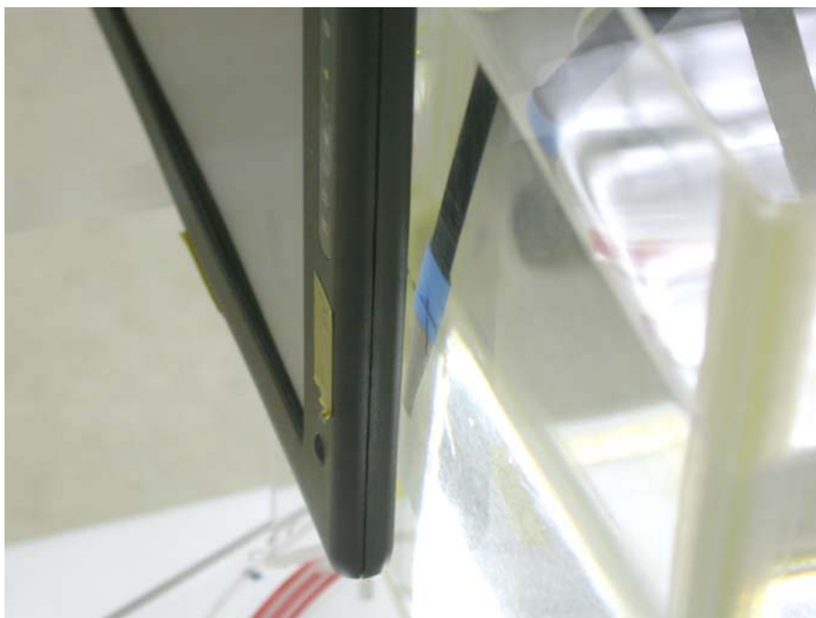
Figure: 7 EUT rear to phantom, 0 mm separation– Zoom In
