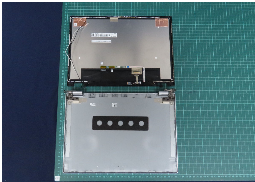
(38) EUT Photo
