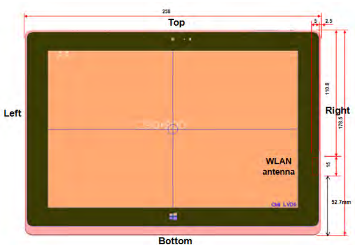
Fig.7 Antenna position (Front view)
