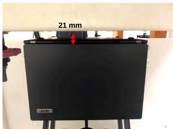
Fig.4 EUT Bottom side (21mm) to flat phantom
