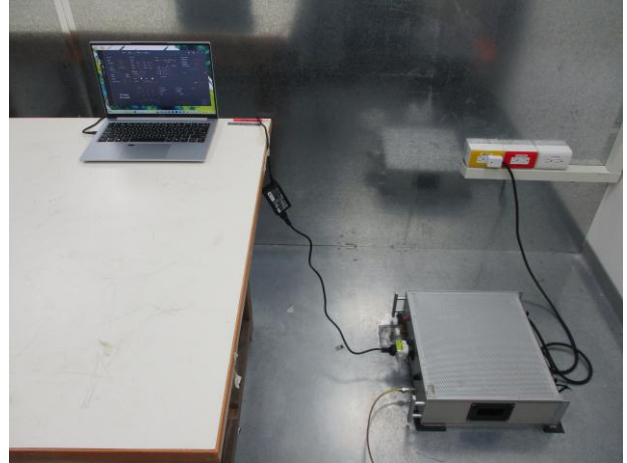
WLAN(2.4G)_Conduction_Setup
