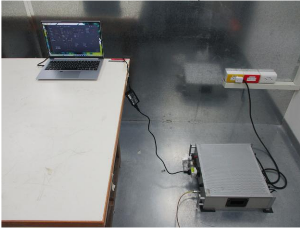
BLE_Conduction_Setup
