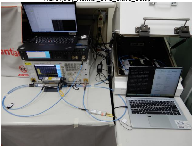
WLAN(5G)_Normal_DFS_Slave_Setup
