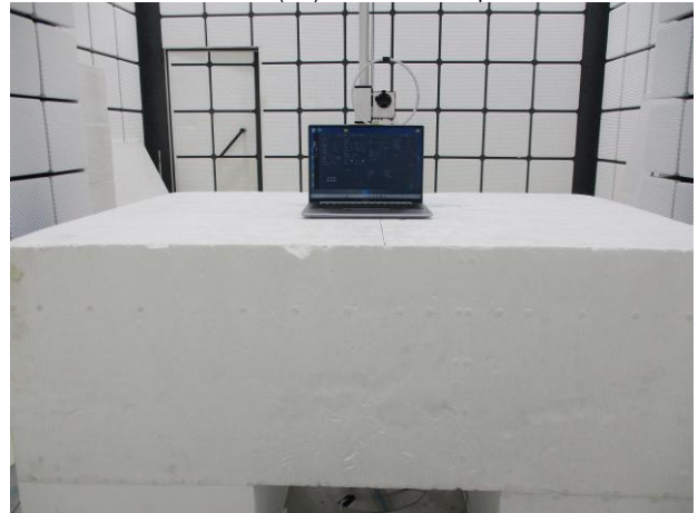
WLAN(5G)_Radiated_Setup
