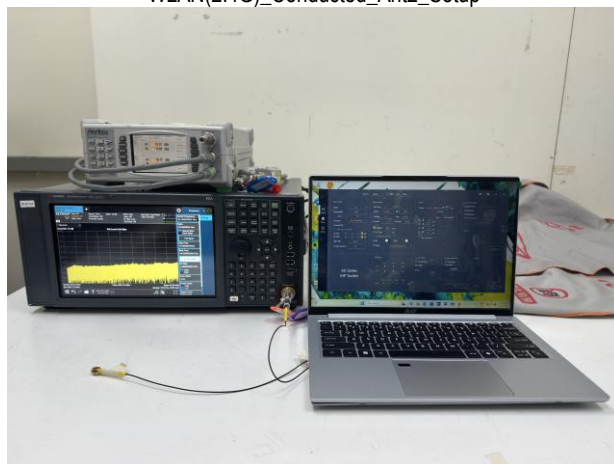
WLAN(2.4G)_Conducted_Ant2_Setup
