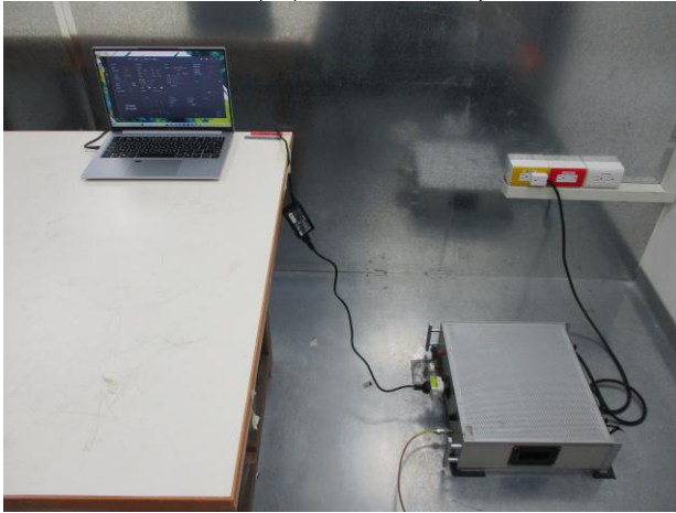
WLAN(5G)_Conduction_Setup
