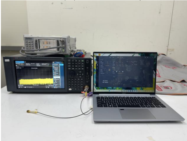
WLAN(5G)_Conducted_Ant2_Setup
