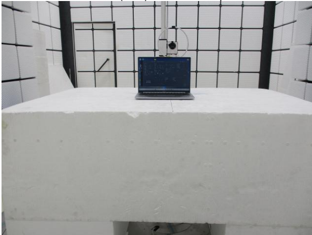
WLAN(5G)_Radiated_Setup
