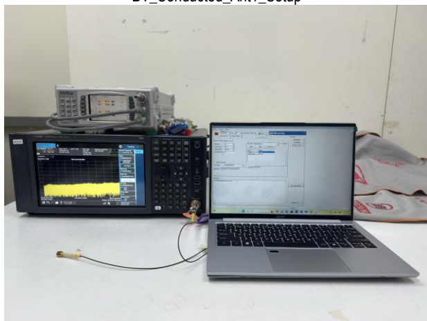
BT_Conducted_Ant1_Setup
