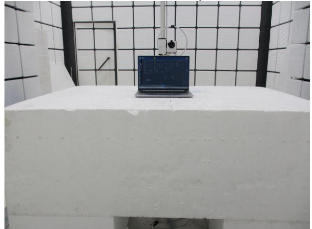
BLE_Radiated_Setup
