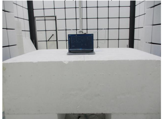
WLAN(5G)_Radiated_Setup
