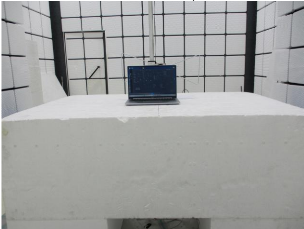
BT_Radiated_Setup
