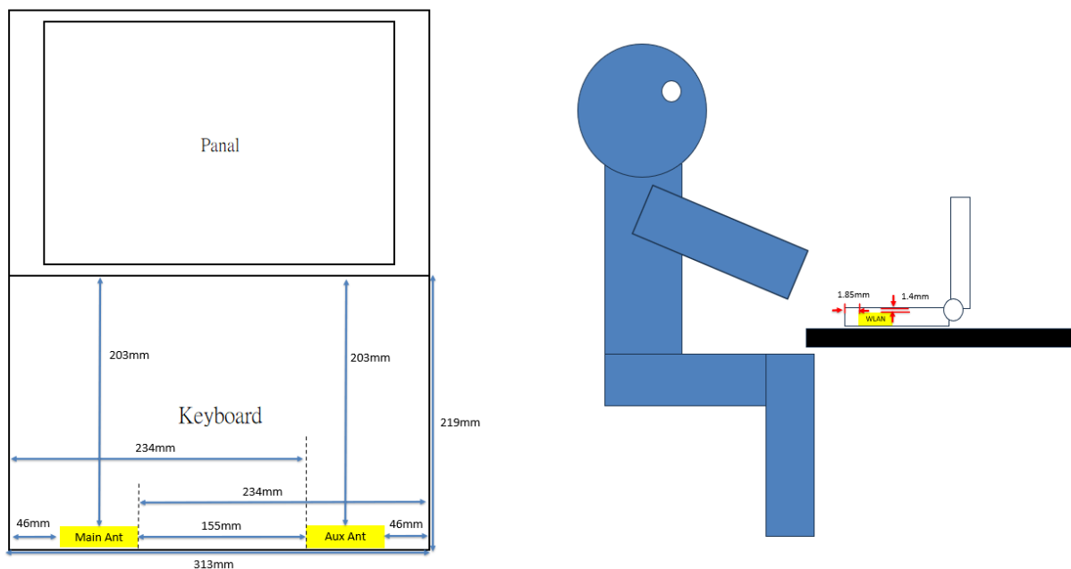
Photograph 5. Antenna position of EUT
