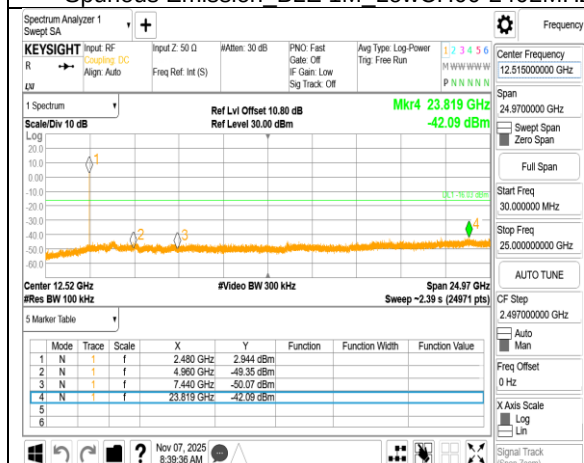
Spurious Emission_BLE 1M_HighCH39-2480MHz
