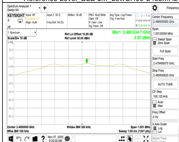
Reference Level BLE 1M HighCH39-2480MHz
