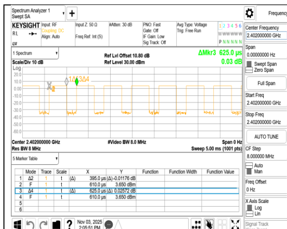
BLE_1M_LowCH00-2402
