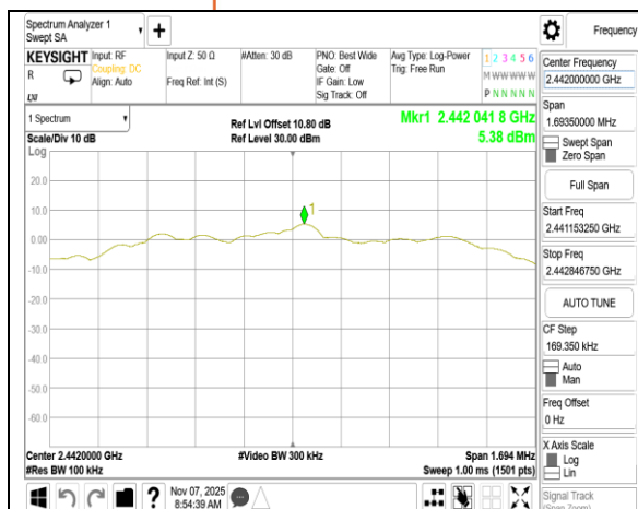
Reference Level BLE 2M_MidCH20-2442MHz
