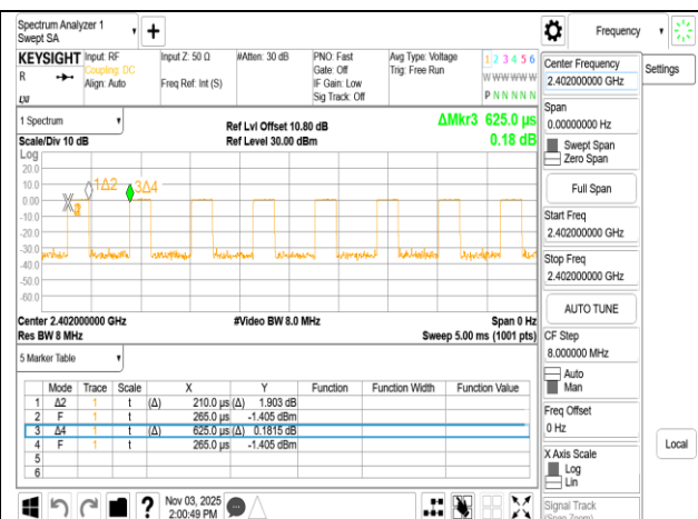
BLE_2M_LowCH00-2402
