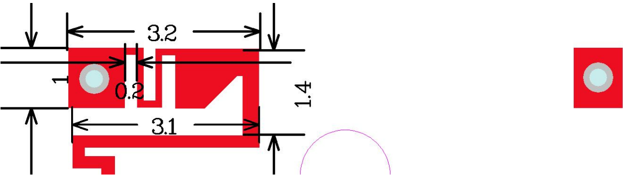
Antenna Photo & Length(mm)
