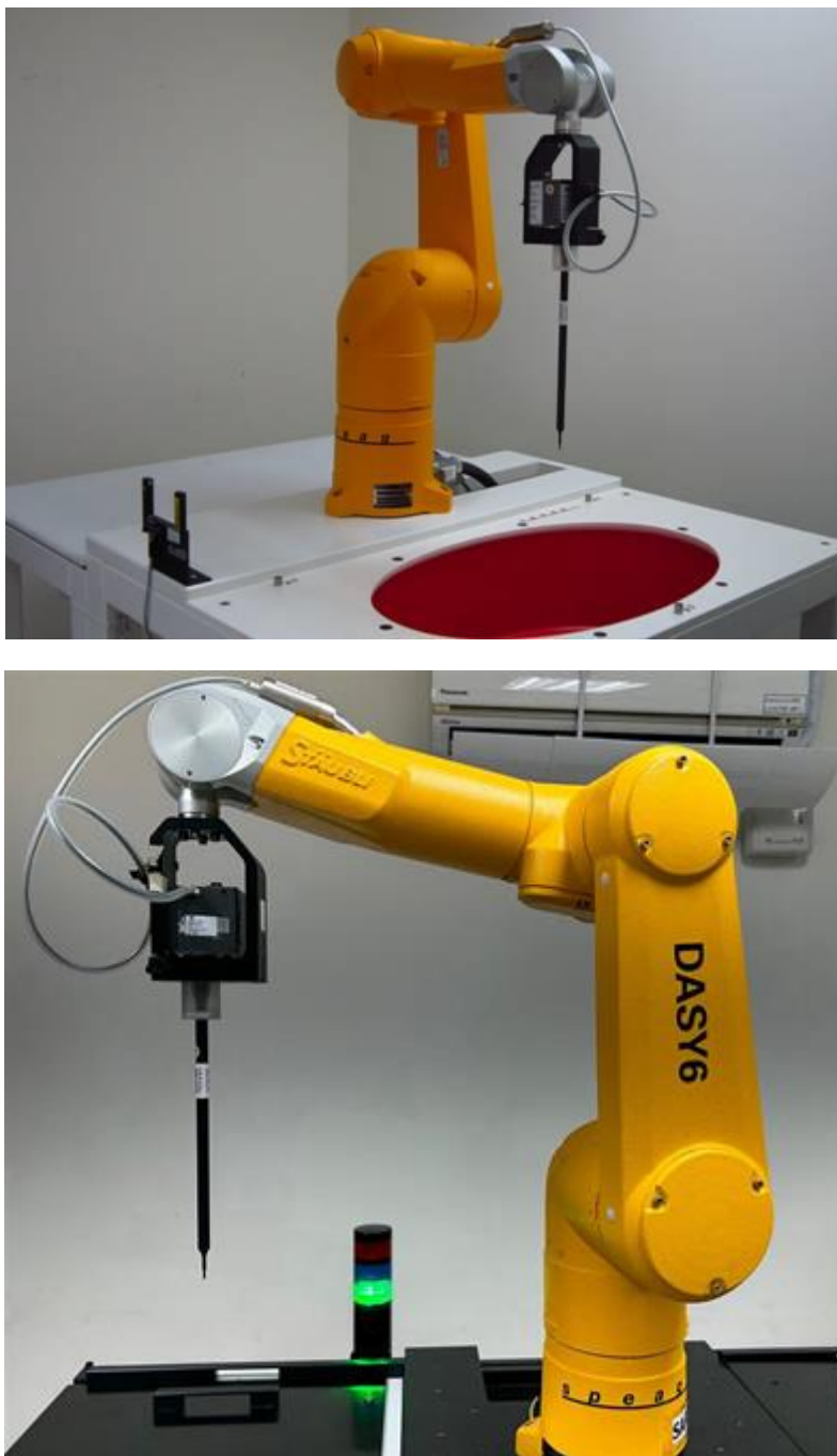
Fig.1 Photograph of the SAR measurement system
