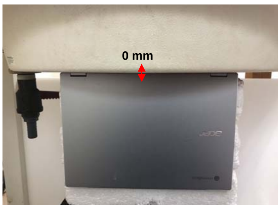
Fig.8 EUT Bottom side (Notebook mode) to flat phantom
