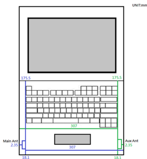
Fig.11 Antenna location of EUT (Tablet mode)
