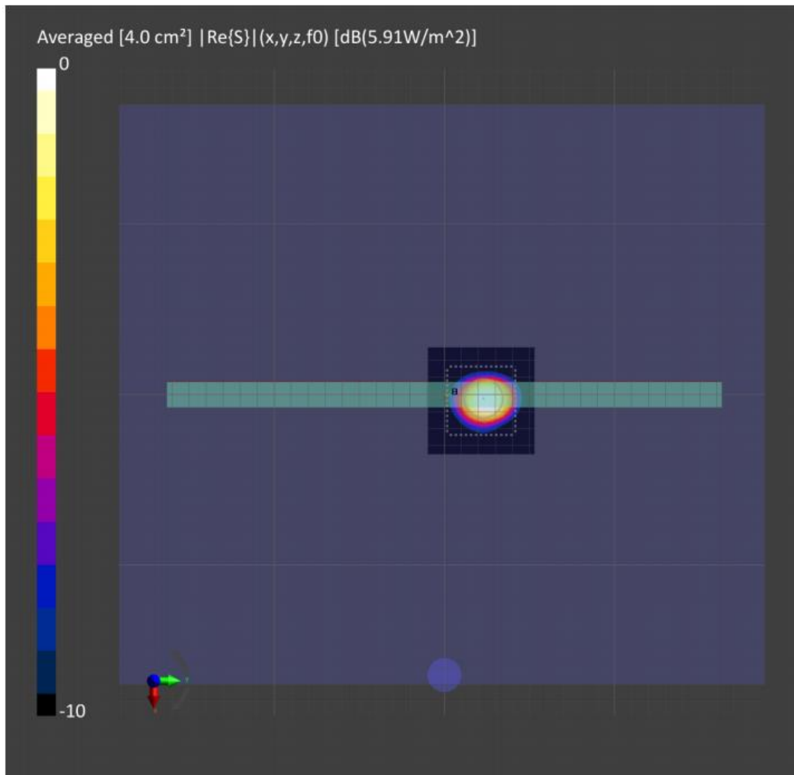
Figure 8-3: 4cm2-averaged power density distribution measured at input.power.limit of 2.36dBm on the back surface for n261 beam 43
