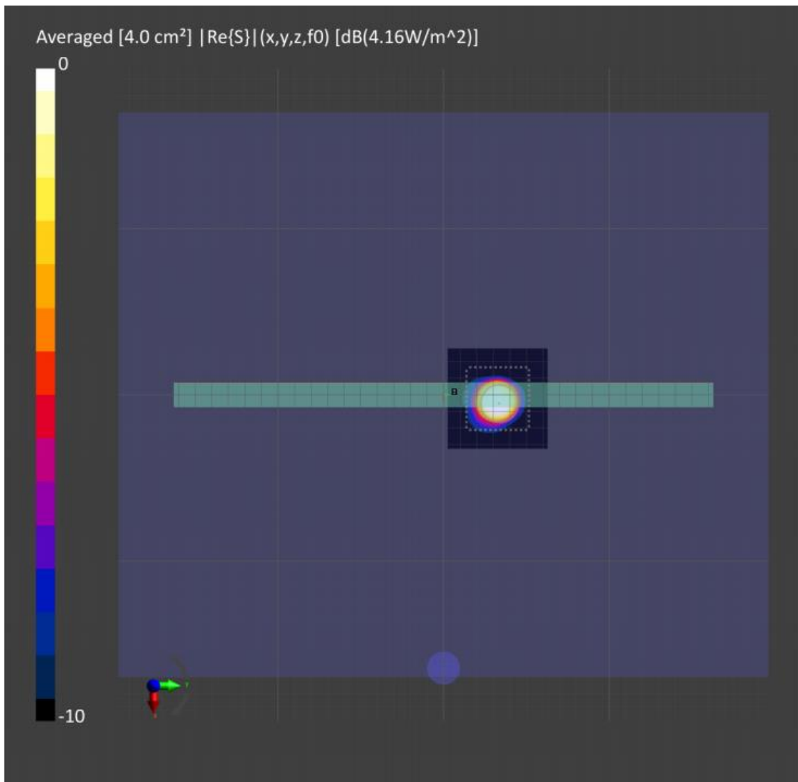
Figure 8-2: 4cm2-averaged power density distribution measured at input.power.limit of 8.22 dBm on the Back for n260 beam 2
