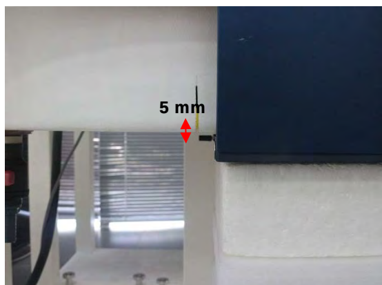
Fig.3 EUT Horizontal-Down to flat phantom
