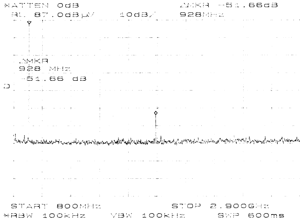
Figure 5 Antenna Emissions
