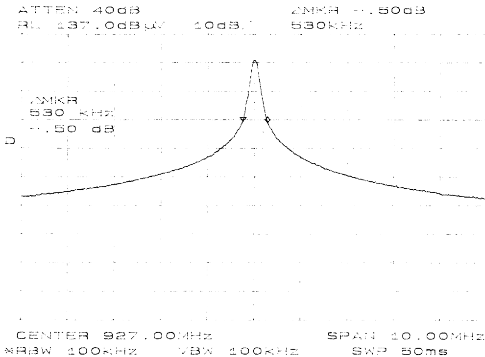
Figure 11 Antenna Conducted Emissions
