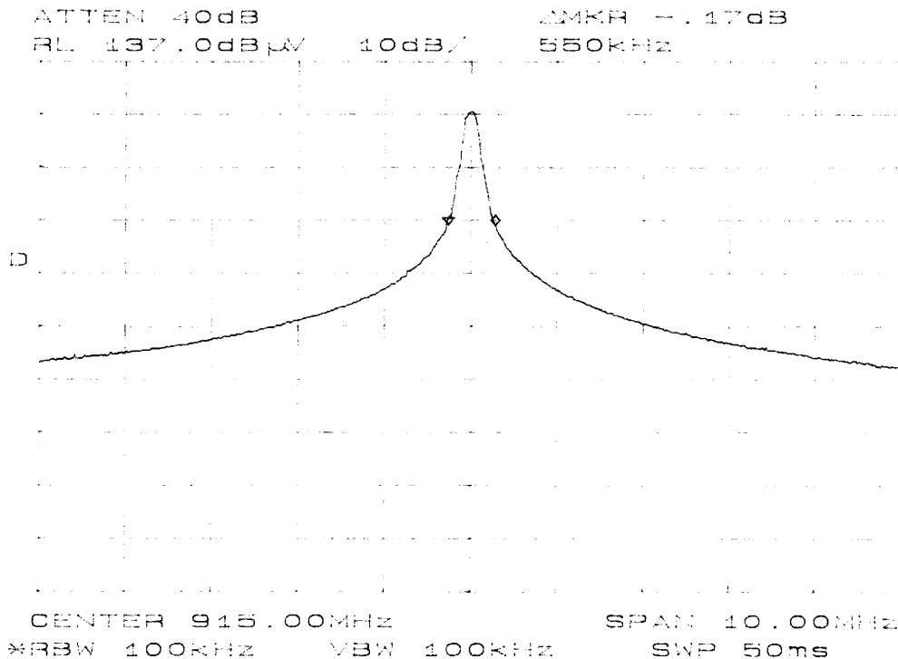
Figure 10 Antenna Conducted Emissions
