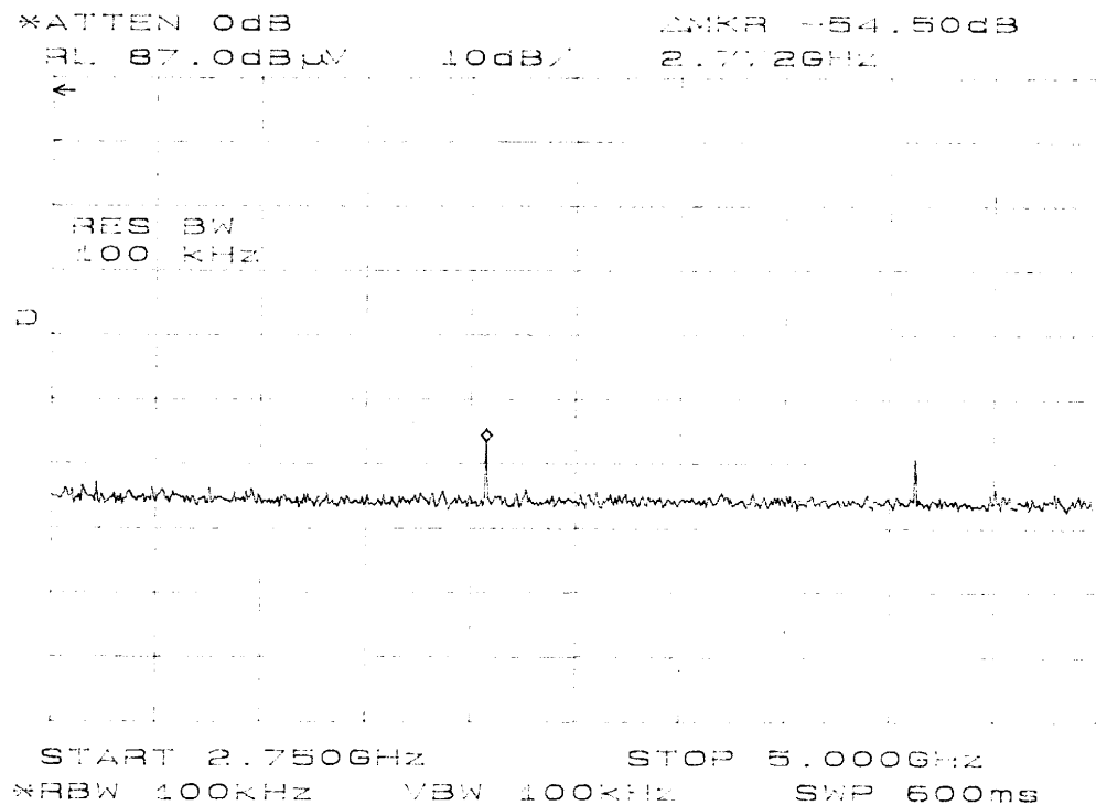
Figure 6 Antenna Emissions
