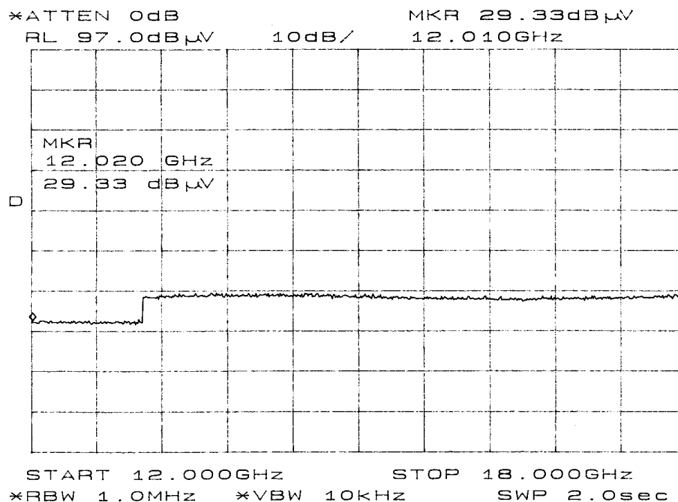
Figure 9 Emissions at Manufacturer Service Antenna Port
