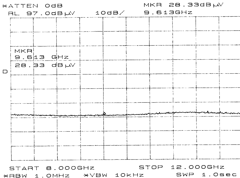
Figure 8 Emissions at Manufacturer Service Antenna Port
