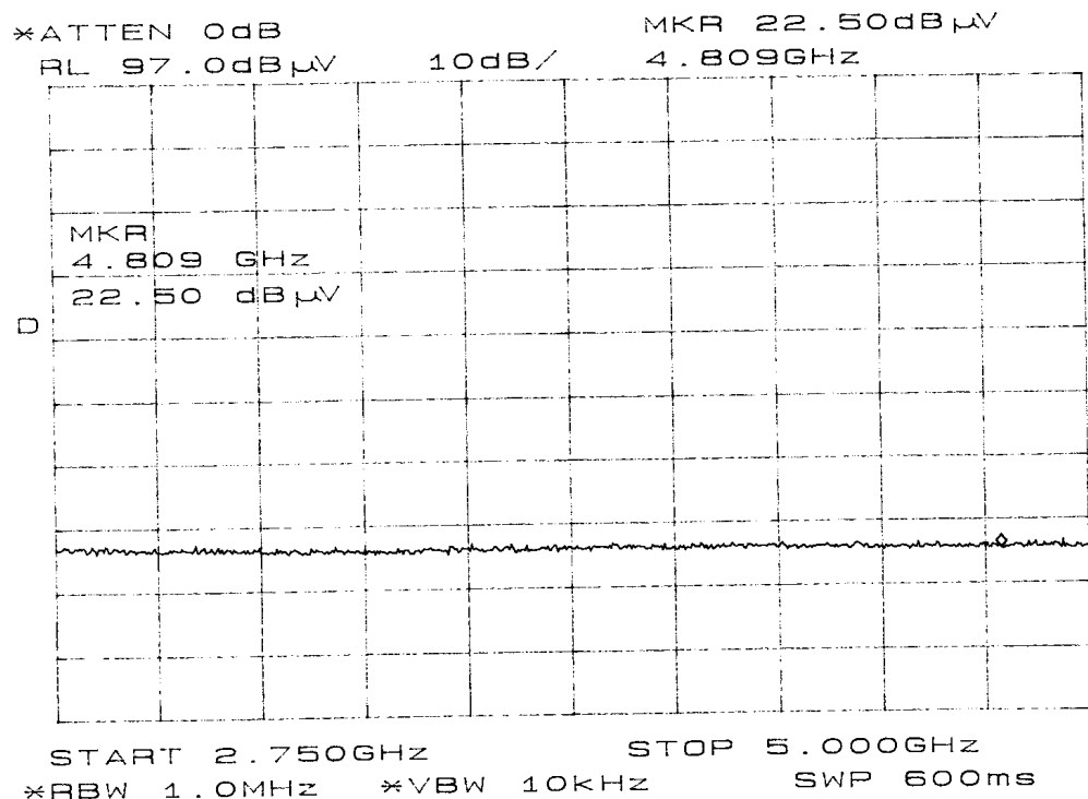
Figure 6 Emissions at Manufacturer Service Antenna Port
