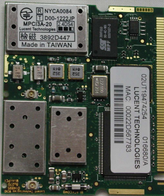
MPC13A-20 Top View (with shields)
