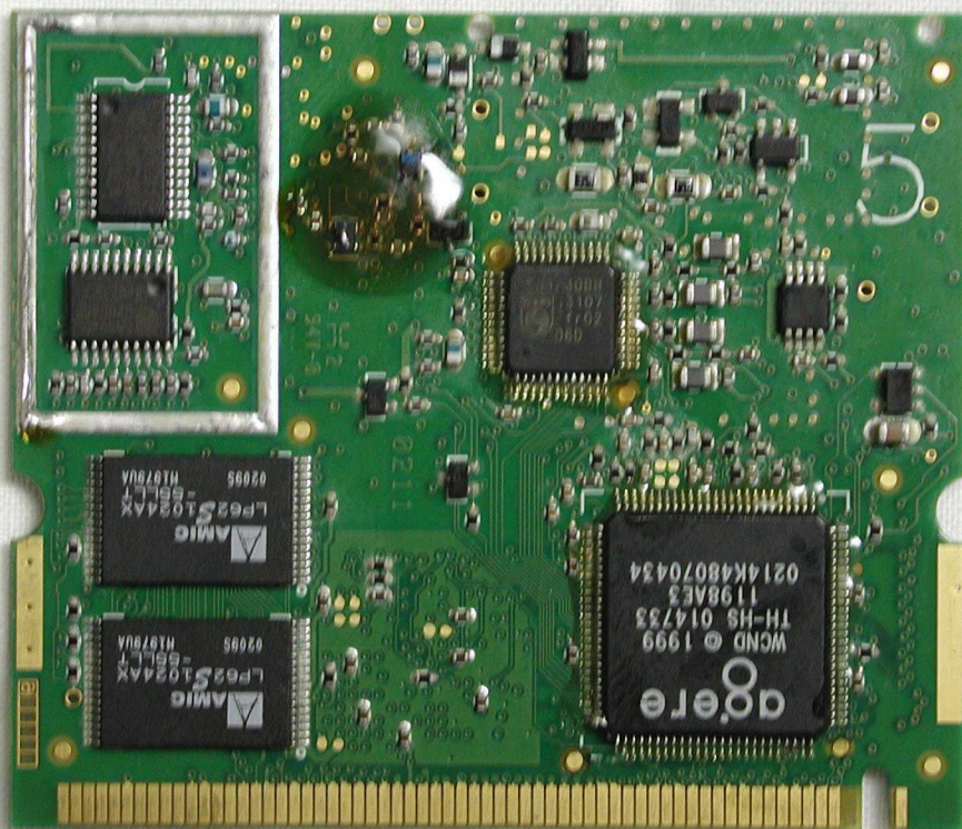
MPC13A-20 Bottom View (shields removed)
