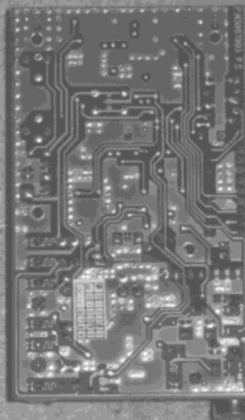
ATLAS Low Power Field Disturbance Sensor. FCC ID: HNA2YUATL PCB, Solder Side.
