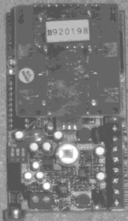
ATLAS Low Power Field Disturbance Sensor. FCC ID: HNA2YUATL PCB, Component side.
