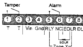
Figure 1: Terminal Block
