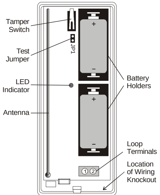
Figure 1: PCB
