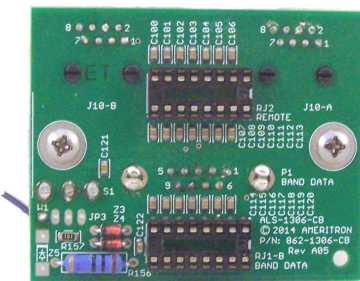
RJ45 Radio Interface Board Component Side
