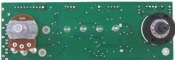
MB2 Meter Board Bottom Side
