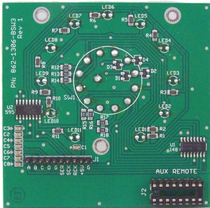
BSW3 Component Side
