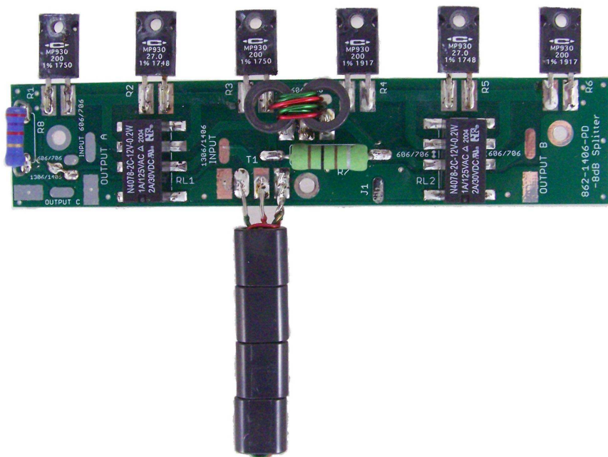
PD8M Power Attenuator and Splitter Board Component Side. Wired for ALS-1406.
