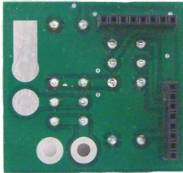
RLY T/R Relay Board Bottom Side
