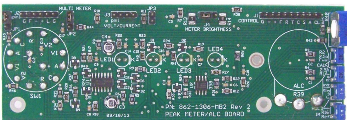
MB2 Meter Board Component Side
