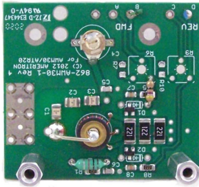
SWR Board Component Side
