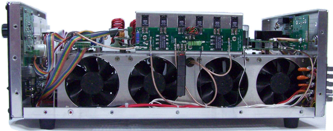
ALS-1406 Right Side with PD8M wired for ALS-1406
