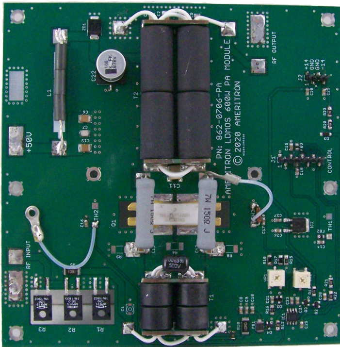
PAM-706 Board Component Side
