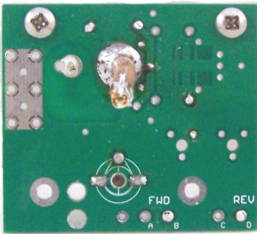
SWR Board Bottom Side
