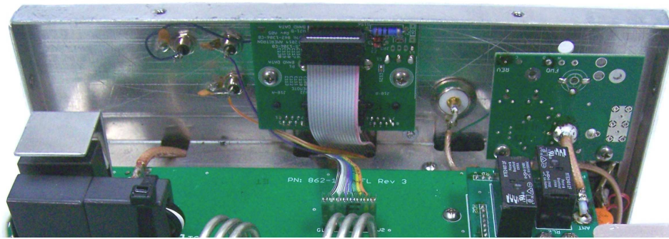
ALS-1406 Back Panel with RJ45 Board and SWR Board
