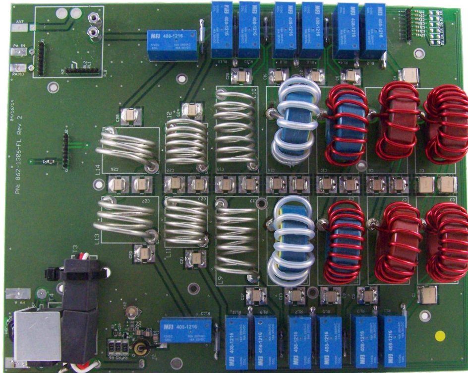
2KWF6 Component Side
