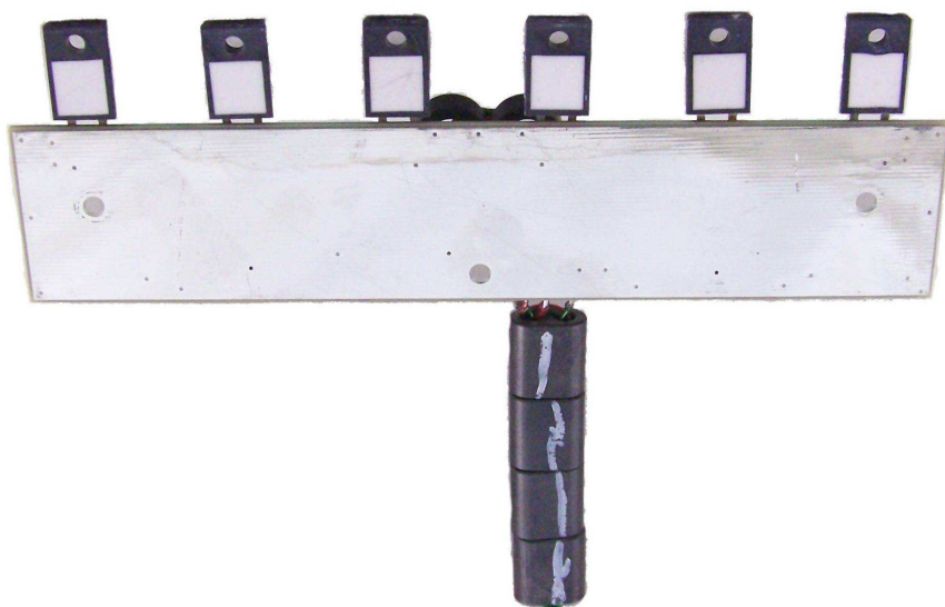
PD8M Power Attenuator and Splitter Bottom Side. Wired for ALS-1406.
