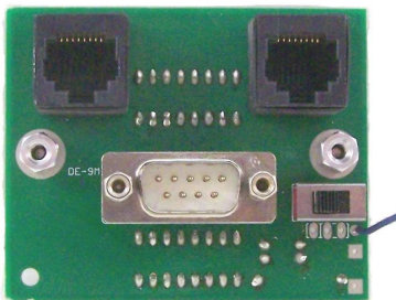
RJ45 Radio Interface Board Bottom Side
