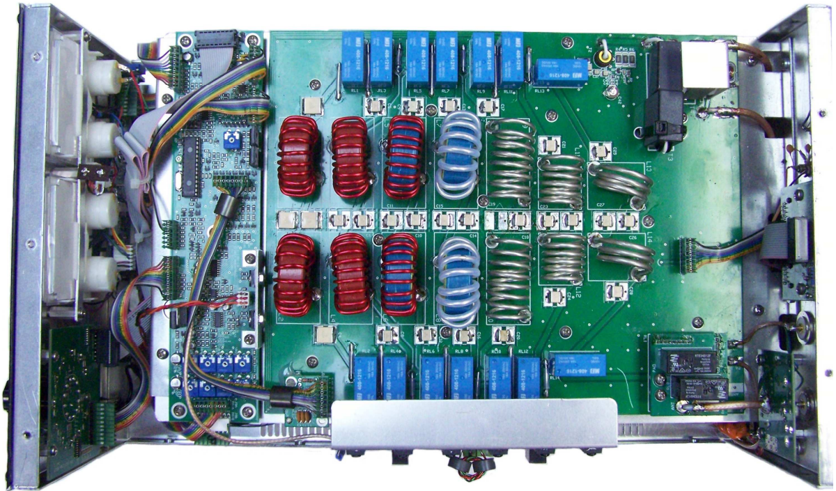
ALS-1406 Top View CB2 Control Board and 2KWF6 Filter Board
