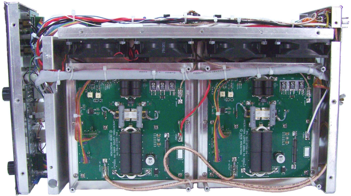
ALS-1406 Bottom View with two PAM-706 Modules
