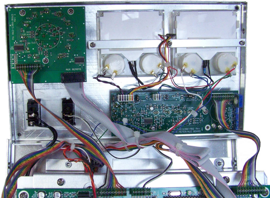
ALS-1406 Front Panel BSW3 Switch Board and MB2 Meter board
