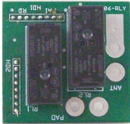
RLY T/R Relay Board Component Side
