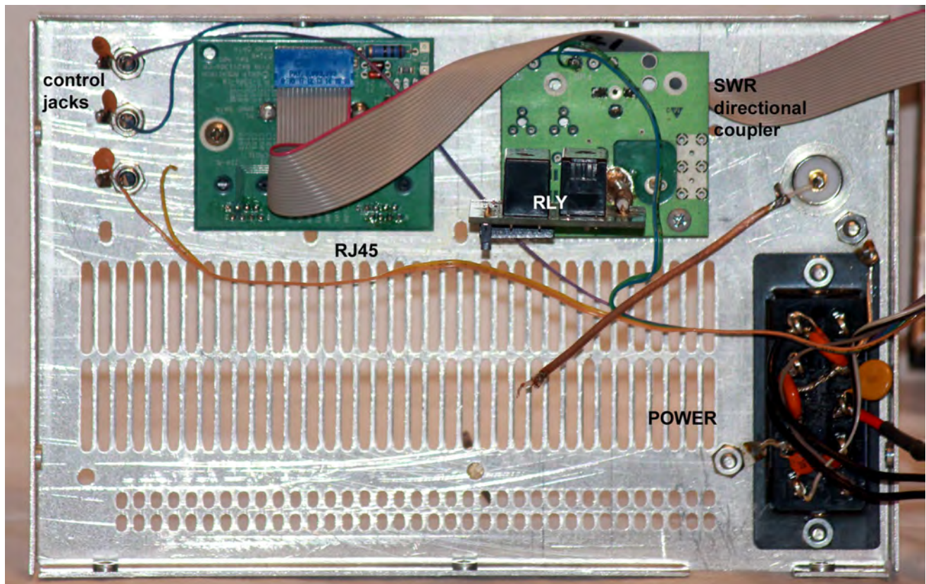
Rear panel
