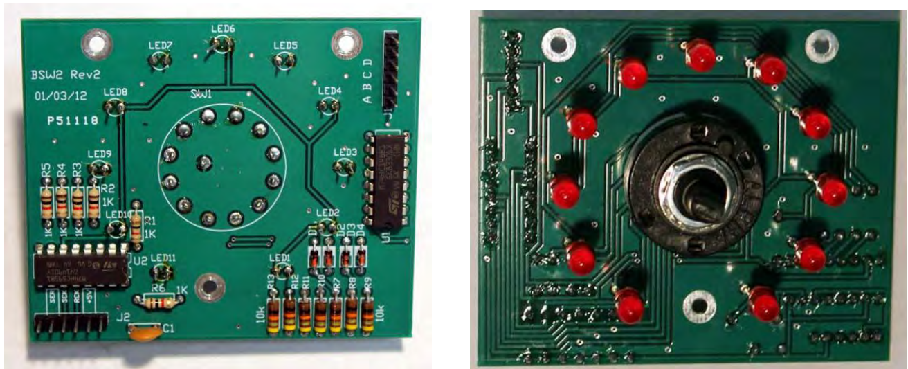
BSW3 (BSW3 top/bottom identical BSW2 Rev2)
