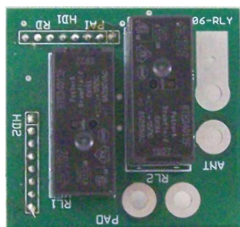
RLY Transmit/Receive Relay Board Component Side
