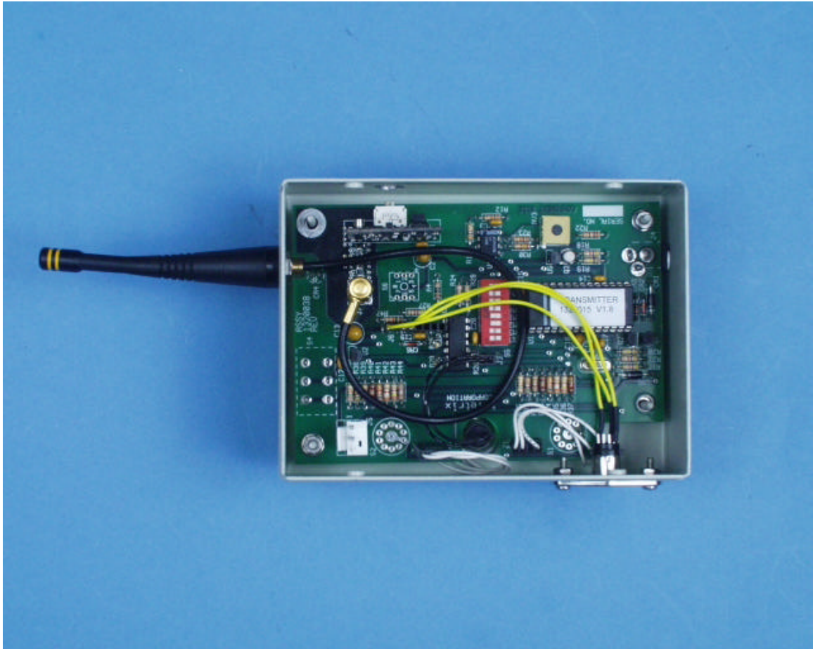
Interior, Component Side
