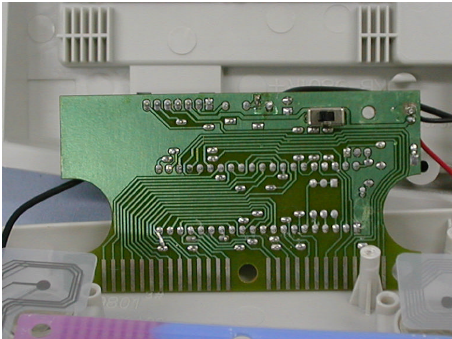
01R9829 Transmitter
