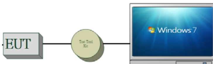
Fig. 2-2 Conducted & Radiated Emission Configuration
