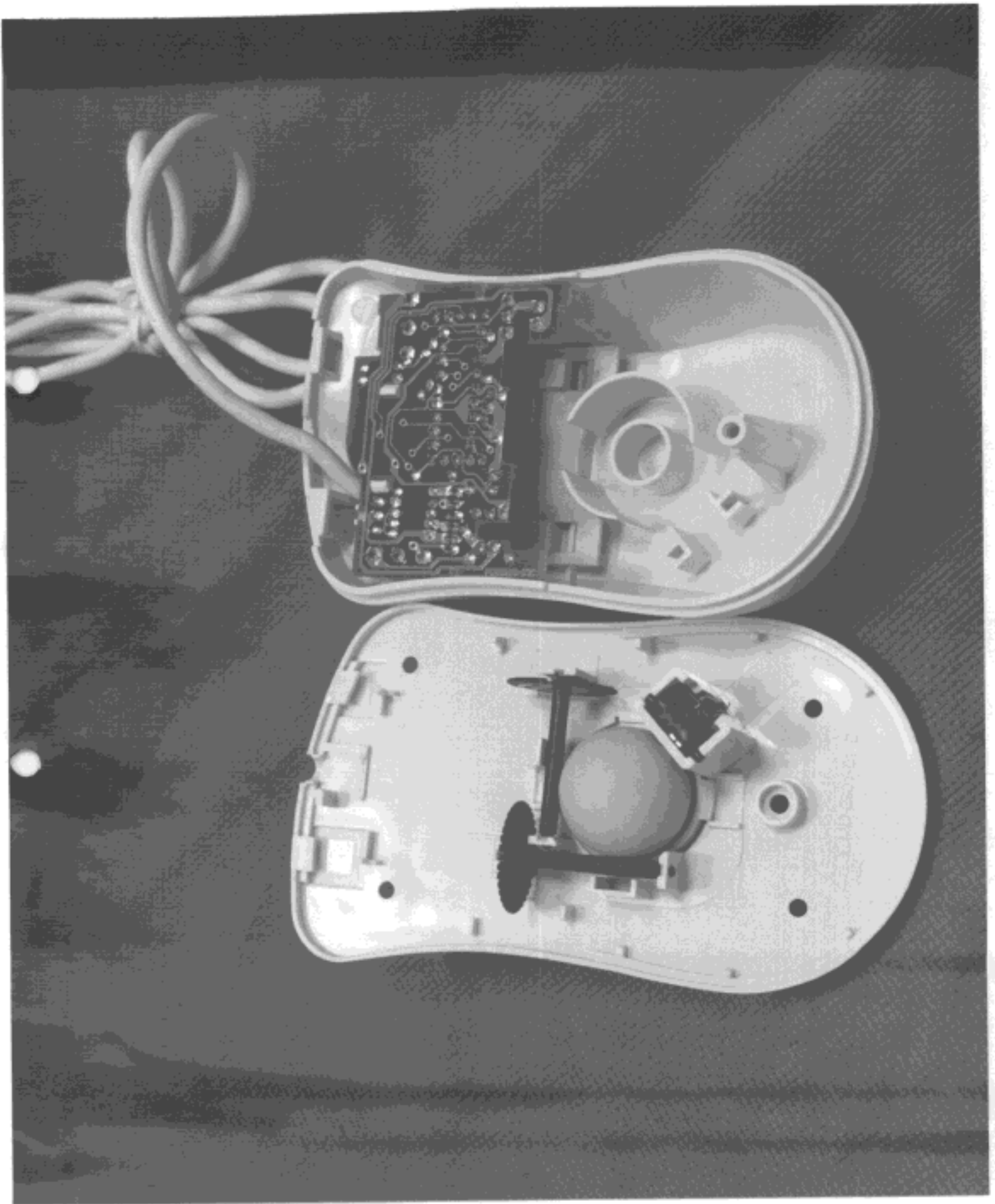
FCC ID: HOXPC98010-13 PHOTO 3. EUT INSIDE VIEW
