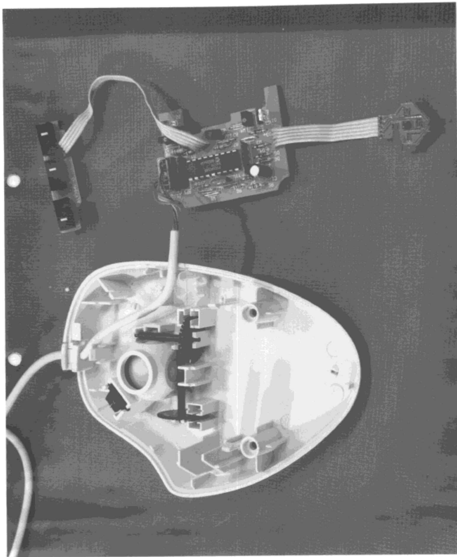
FCC ID : HOXPC98010-18 PHOTO 4. EUT INSIDE VIEW
