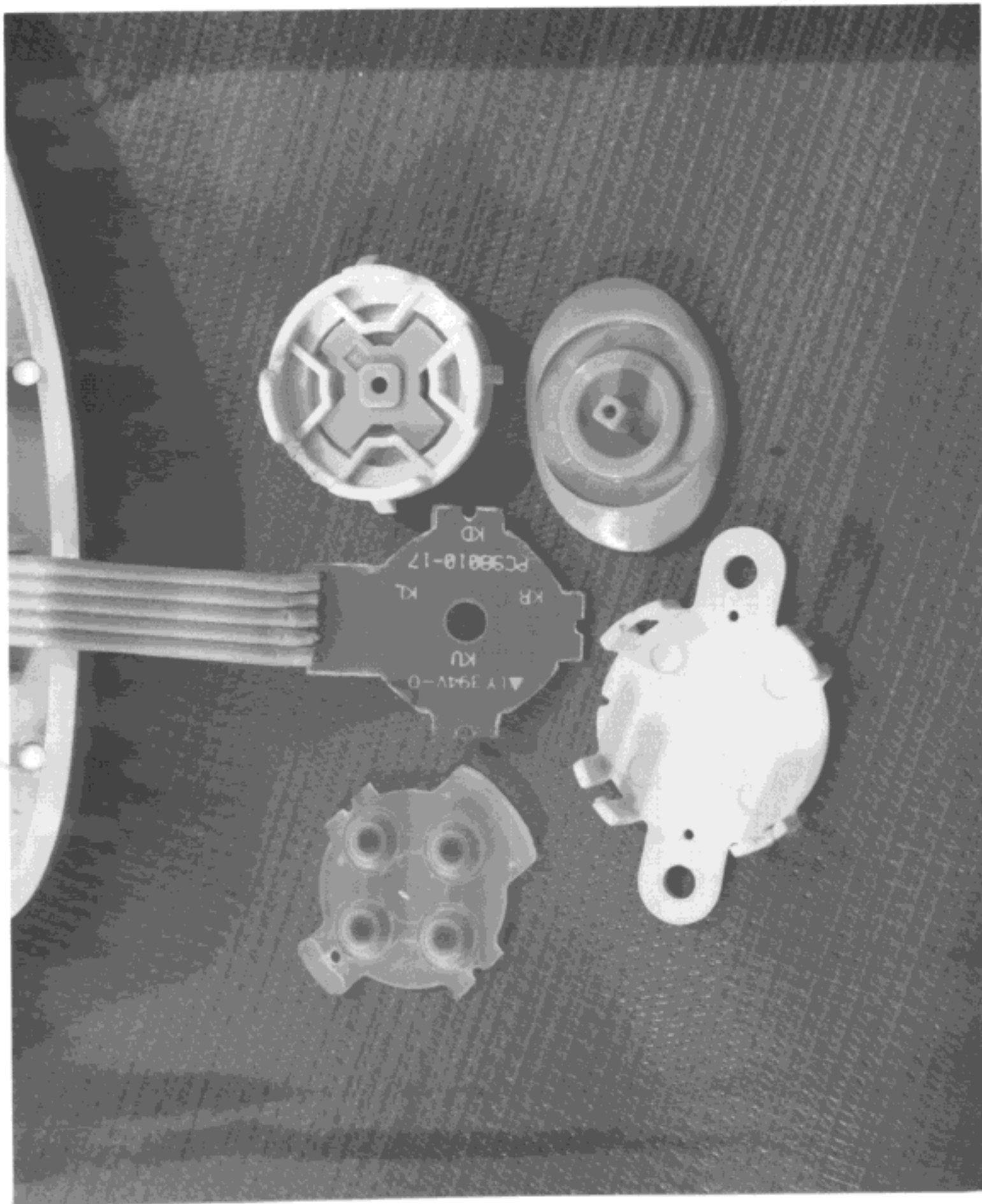
FCC ID: HOXPC98010-18 PHOTO 5. EUT INSIDE VIEW
