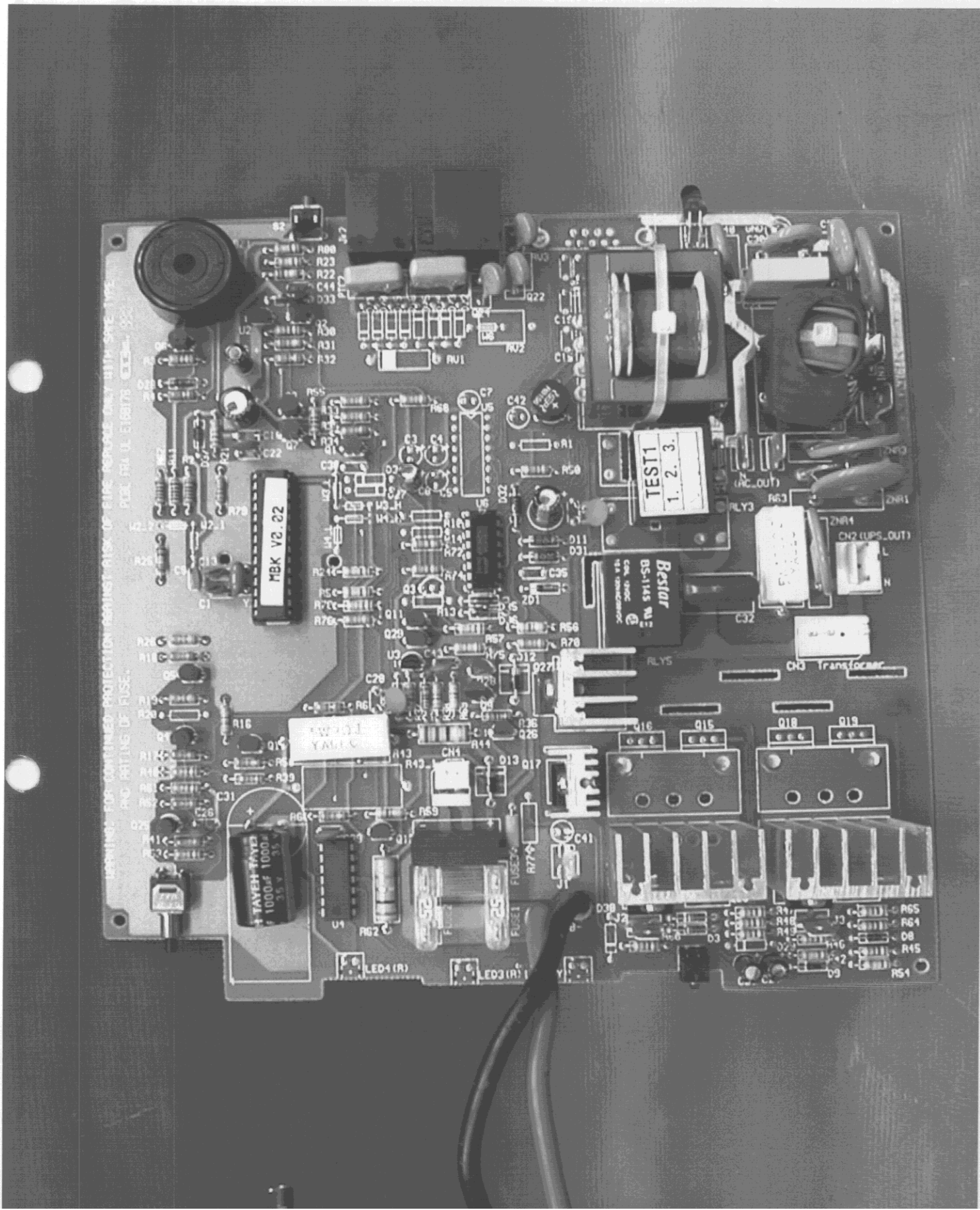
PHOTO 5. EUT COMPONENT SIDE VIEW (MBK 320)
