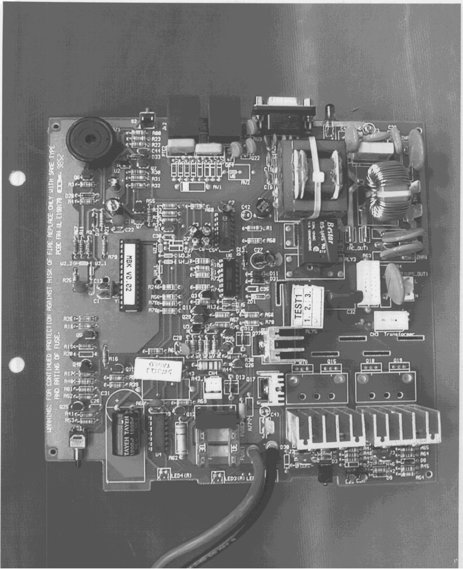
PHOTO 11. EUT COMPONENT SIDE VIEW (MBK 520)
