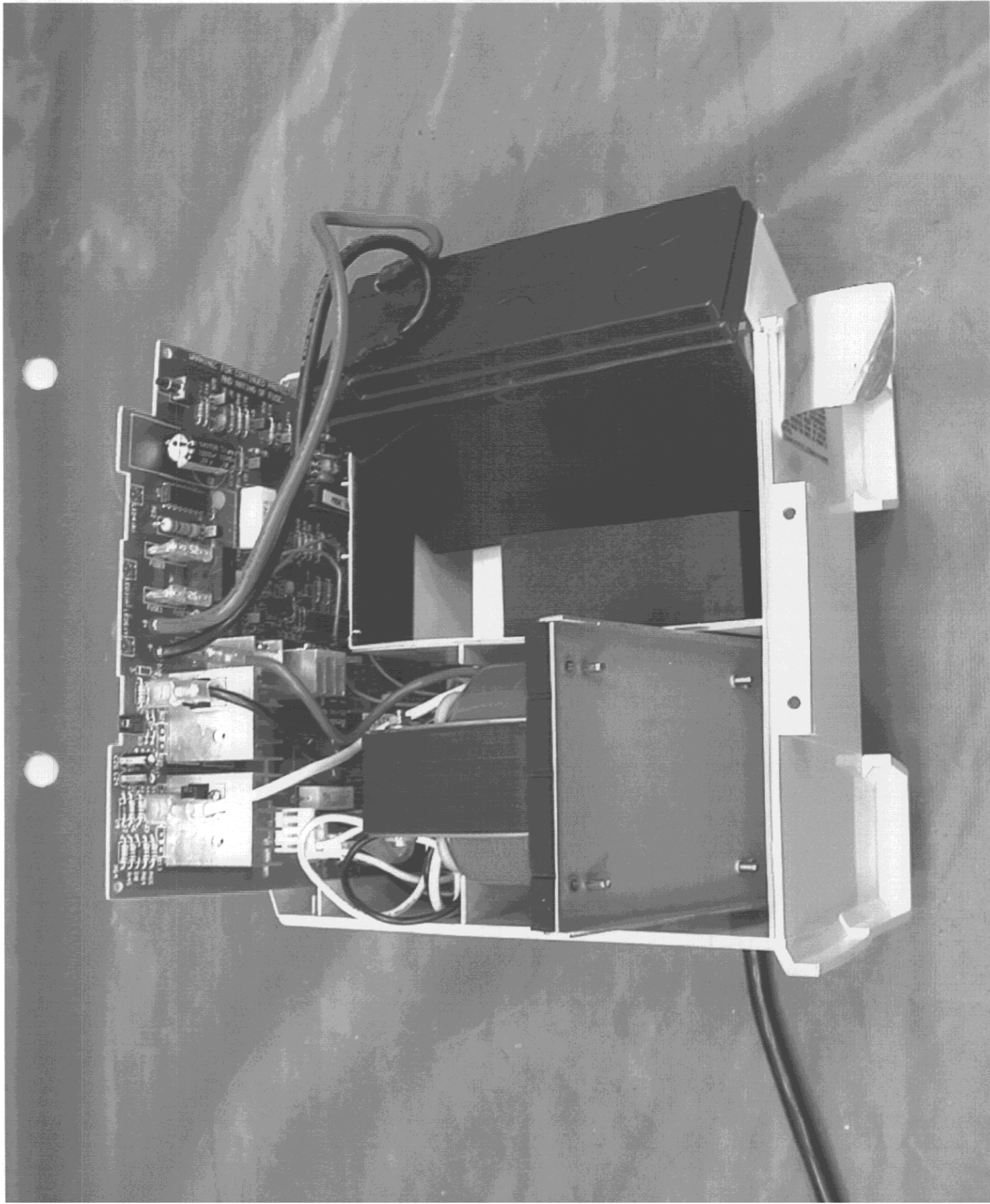
PHOTO 4. EUT INSIDE VIEW (MBK 320)
