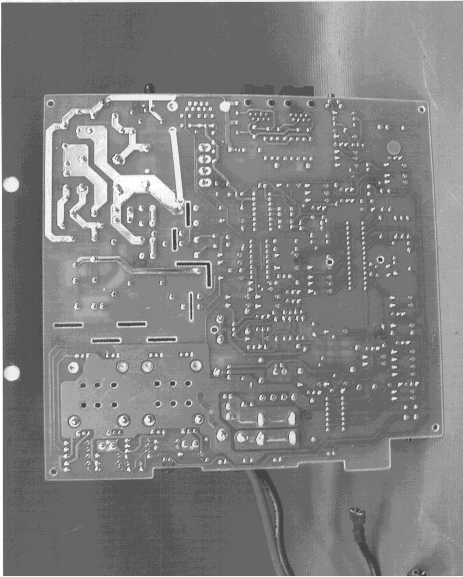
PHOTO 6. EUT SOLDERING SIDE VIEW (MBK 320)
