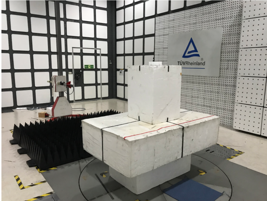
Photograph 4: Set-up for Radiated Emissions (Back View 3)
