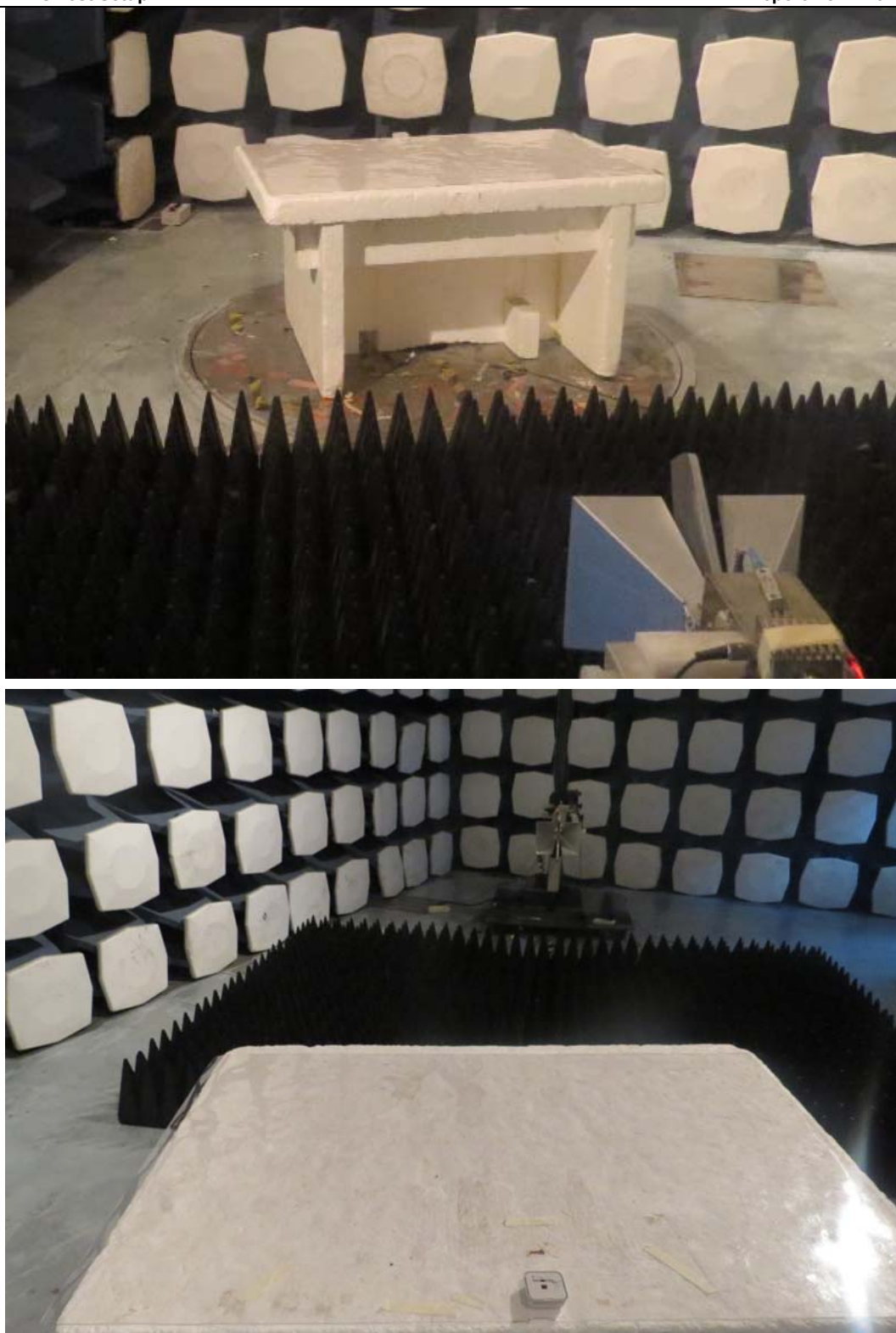
Picture 1 Radiated Emission Test Setup
